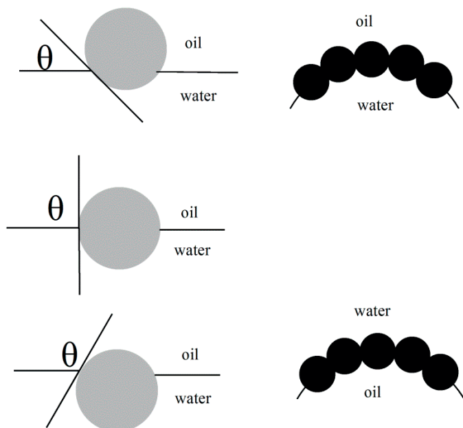
Figure 5. Schematic of particle stabilization for oil-in-water (o/w) and water-in-oil (w/o) Pickering emulsions.
