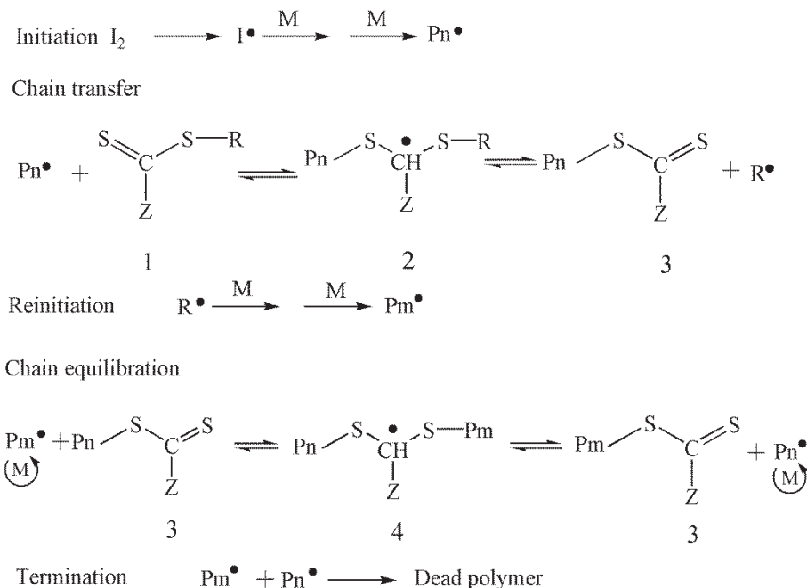
Figure 12. Equilibria of RAFT polymerization.
