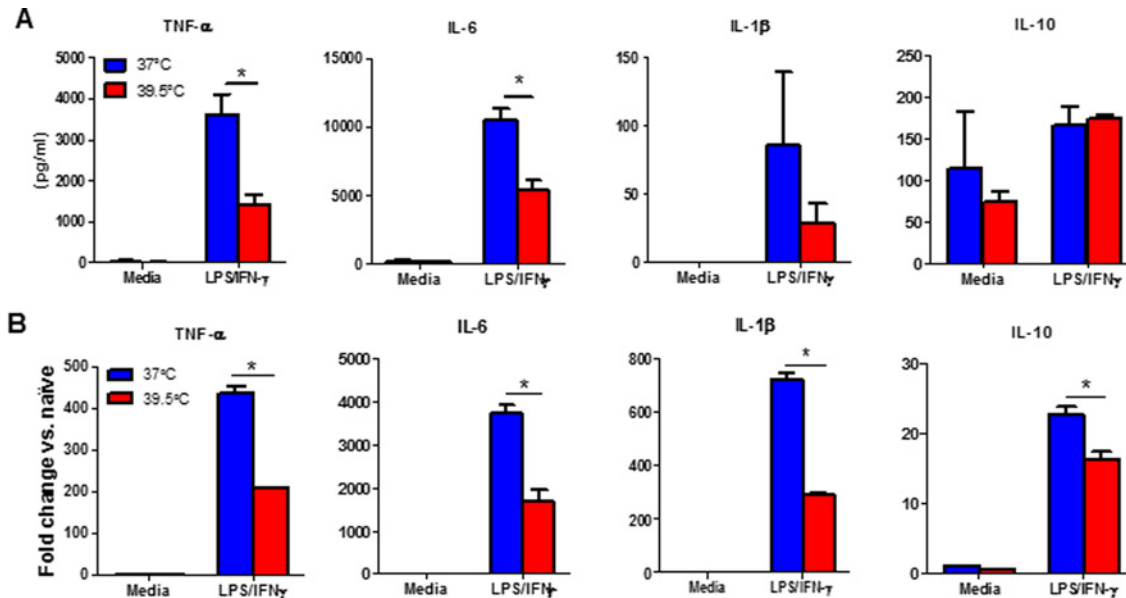
Fig 4. In vitro heat treatment inhibits LPS-induced cytokine production by activated macrophages. (A-B), BALB/c mice were injected intraperitoneally with 10 µg of LPS. Peritoneal macrophages were harvested 3 days post LPS injection, recovered overnight and re-stimulated ( 2 \times 10^5 /well) with LPS (100 ng/mL) and IFN- \gamma (25 U) at 37°C or 39.5°C for 6 hours to determine TNF- \alpha , IL-6, IL-1 \beta and IL-10 production by ELISA (A) or re-stimulated ( 1 \times 10^6 /well) for 4 hours to measure TNF- \alpha , IL-6, IL-1 \beta and IL-10 mRNA expression by quantitative real-time PCR (B). The results are presented relative to GAPDH and baseline expression in unstimulated cells at 37°C. Cells from each treatment condition were pooled from 2–4 mice and measured in triplicate. Data are mean \pm SD. Data are representative of three independent experiments. * p < 0.05 , paired Student t test and repeated-measures two-way ANOVA.
