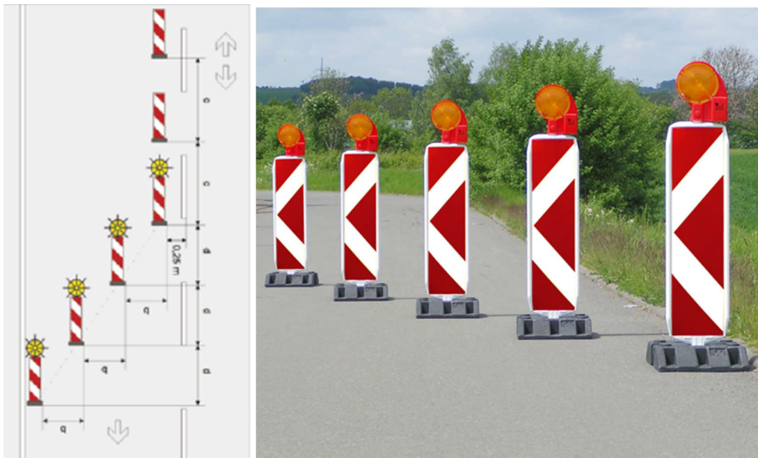
Figure 28. Running lights; Source: BRoWSEr-Project, CEDR, 2015 (left), www.rosa-moser.at (right)
