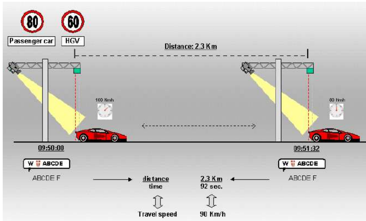
Figure 21. Scheme of average speed control. Source: Stefan ( 2006)
