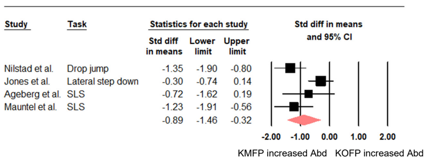
Figure 6. Difference in 3D knee abduction between individuals with a knee medial-to-foot position (KMFP) or a knee over foot position (KOPF).
