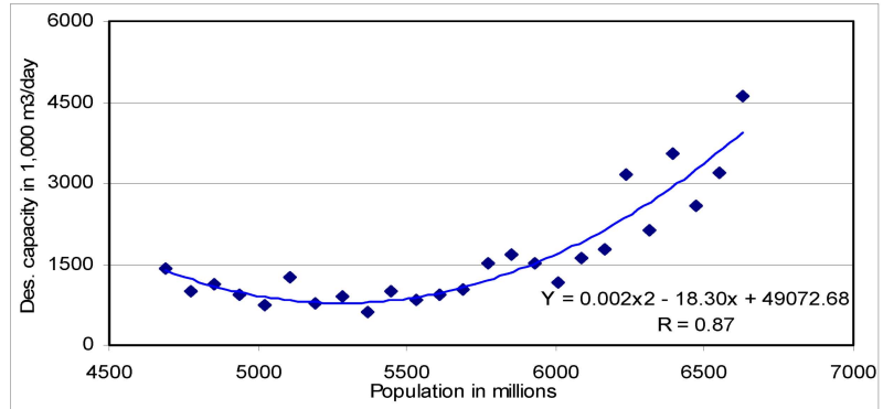
Fig. 5. World daily desalination capacity versus world population
