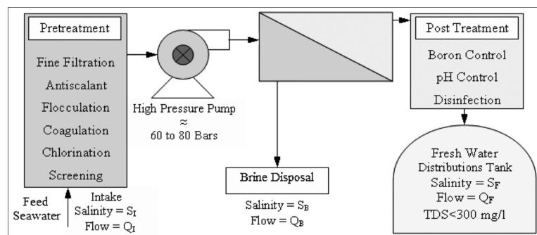
Fig. 1. Reverse osmosis seawater desalination plant typical scheme showing input/output and different stages of treatment.
