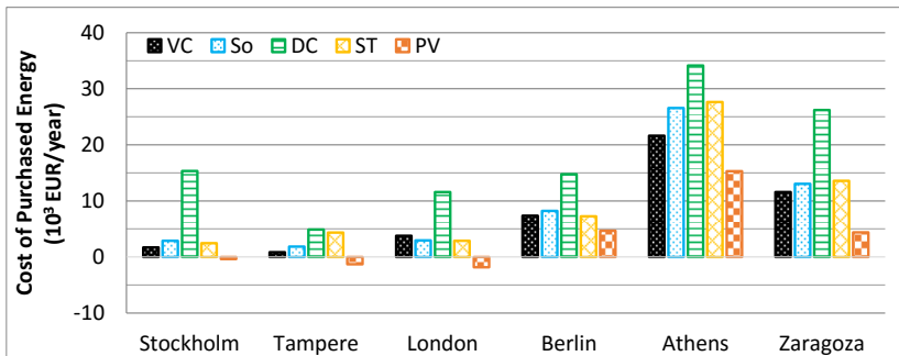
Fig. 4 Annual energy costs for each investigated cooling systems.
