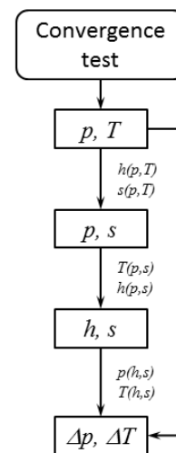
Figure 3. Convergence test flow chart
