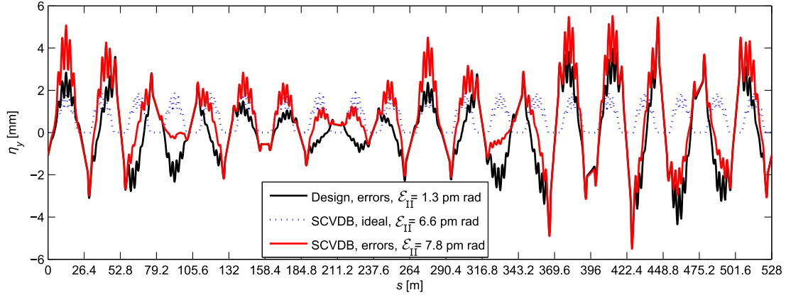
(b) Resulting vertical emittance, \varepsilon_{II} = 8 \text{ pm rad} scaling.
