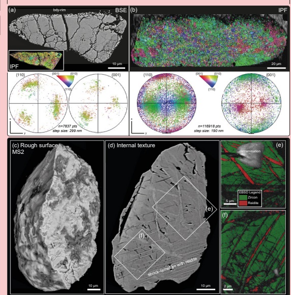
Figure 3. EBSD analyses: granular zircons with baddeleyite rim(?) from (a) melt-bearing impact breccia (thin section) and (a) impact-melt (separate), yields three main clusters with high angle arrangements towards each other – coinciding between {001} and {110} pole projections (fig. 3a and 3b; IPF colours represent neoblast orientations), indicative of FRIGN zircon. BSE-images on rough surface (c) and internal texture (d) of zircon MS2 from the melt-bearing impact breccia (3). EBSD analysis indexing reidite within several intersecting planar shock-lamellas (fig. 3e-f).
