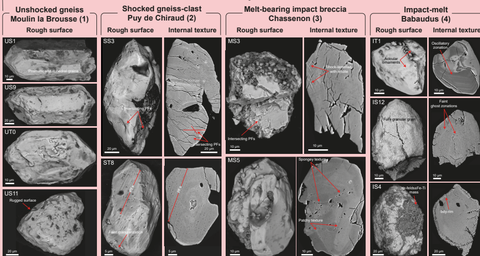
Figure 2. SEM-BSE images of zircons in: 1) control sample and (2-4) the impactites. 1) No shock features are present, mainly prismatic, euhedral grains with rugged surfaces. 2) Well defined intersecting PFs (SS3) and PFs (ST8). 3) Shock lamellae with reidite (MS3) and an altered grain with patchy and spongy texture (MS5). 4) Rare grain with oscillatory zonations and acicular ornaments (IT1), fully granular grain with preserved ghost zonation (IS12) and a fully granular grain with a baddeleyite rim, partially covered with a quartzfeldspathic(±Fe-Ti oxides) microcrystalline mass (IS4) similar to the groundmass of the impact-melt.
