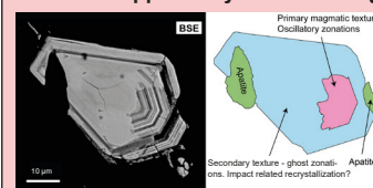
Figure 4. Zircon from (3). One of several grains with recrystallized domains and ghost zonation (blue). Here, the primary magmatic texture is also preserved (pink). Impact related (?) recrystallization fronts has likely experienced a reset of the U-Pb system.
