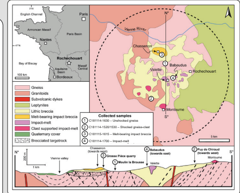
Figure 1. Simplified geological map of the Rochechouart impact structure – displaying various target bedrock, impactites and location of the investigated samples (1-4). Modified after [3] and [6].
