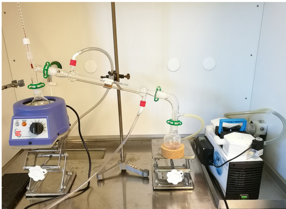
Figure 3: Photo of the glassware of the distillation setup.
