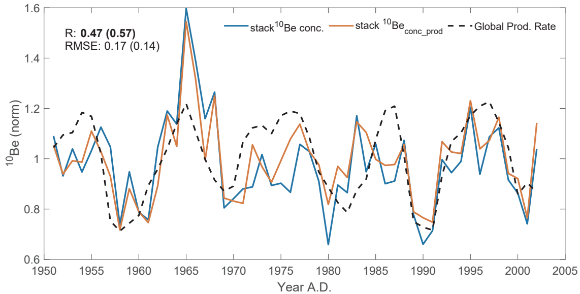
Figure 16. Comparison of the global average production rate (dashed black), the stack of ^{10}\text{Be} concentrations (blue) and the stack of ^{10}\text{Be}_{\text{conc\_prod}} (red) for the period 1951-2002 (see text). Values in the brackets are R and RMSE values between ^{10}\text{Be}_{\text{conc\_prod}} and global averaged production rates. The bold R-value indicates the significant result at p < 0.05 tested by a t-test adjusted for autocorrelation of data (Hu et al., 2017). All data are linearly detrended before analysis.
