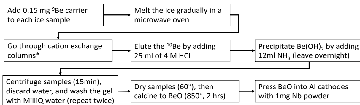
Figure 9. Flowchart showing the procedure for extracting the ^{10}\text{Be} from ice samples for AMS measurements. *denotes as Bio-Rad Poly-Prep ® pre-filled chromatography cation columns AG 50W-X8 resin 100-200 mesh hydrogen form 0.8x4 cm.
