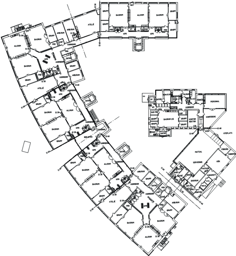
Figure 15. School Ve, ground floor layout of the four-storey building. School Ve only occupied the ground floor.
