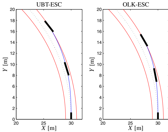
Fig. 2. Geometric trajectories for UBT-ESC and OLK-ESC, with \eta = 100 , \gamma_u = 1 , and R = 30 m. The black bars represent the vehicle position and heading direction for the initial, half-way, and final time-instant.
