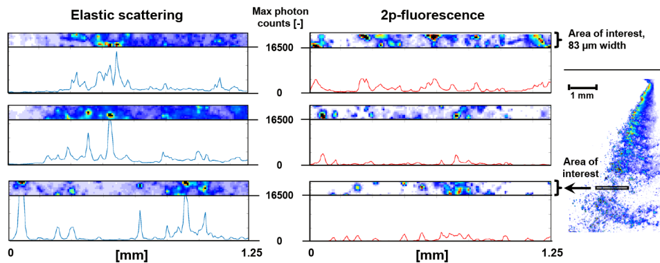
Fig. 8. Optical signals comparison between elastic scattering and 2p-LIF light sheet imaging. The area of interest is located at 4 mm below the nozzle tip as shown in the image on the right. Each image corresponds to independent injection events. It is observed here that the Mie scattering image is locally affected by strong reflections that saturate the 14 bit camera. On the contrary the 2p-LIF signal does not show those unwanted intensity peaks.
