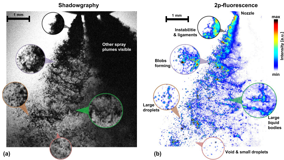
Fig. 6. Image results comparison between shadowgraphy in (a) and 2p-LIF light sheet imaging in (b) for a 6 holes GDI spray injected at 200 bars liquid pressure and recorded at 200 \mu s. The two images have been recorded with the exact same camera system and operating conditions. While the shadowgraph image shows blurred liquid structures; the droplets, liquid blobs, ligaments and voids are clearly observable in the \times 2 zoomed areas of the 2p-LIF image.
