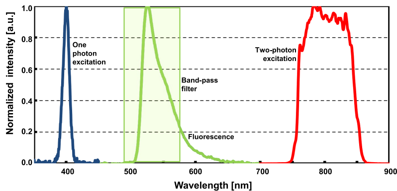
Fig. 4. Spectra of the one-photon excitation at 400 nm, the fluorescein emission and the two-photon excitation centered at 800 nm. To generate the 400 nm excitation pulse, the 800 nm laser beam is frequency doubled by inserting a BBO crystal.
