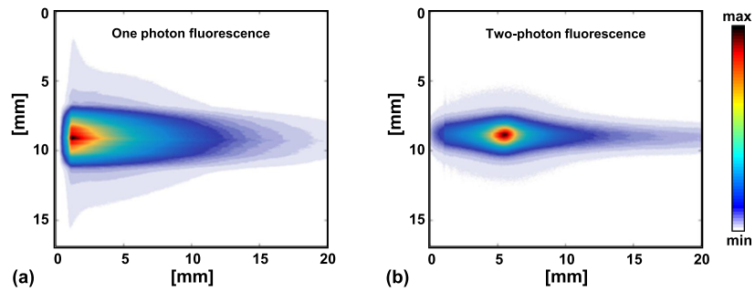
Fig. 1. Comparison between single-photon (a) and two-photon (b) excitation processes for a beam crossing a water solution containing diluted fluorescein dye. In (a), the dye is excited at 450 nm using a CW diode laser. In (b) femtosecond pulses generated by a titanium-sapphire femtosecond laser are used to excite the water solution. In this example the incident beam is focused by a cylindrical lens of +50 mm focal length.
