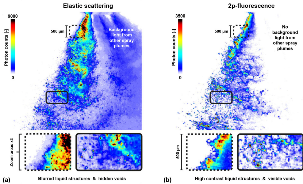
Fig. 7. Light sheet imaging comparison between elastic scattering in (a) and 2p-LIF light sheet imaging in (b) for the 6 holes GDI spray injected at 200 bars liquid pressure and recorded at 200 μs. The two images have been recorded with the same camera system but corresponds to independent injection events. It is seen from the ×3 zoom areas that 2p-LIF provides images with limited blur allowing the visibility of liquid structures which are not observable with the elastic scattering scheme.
