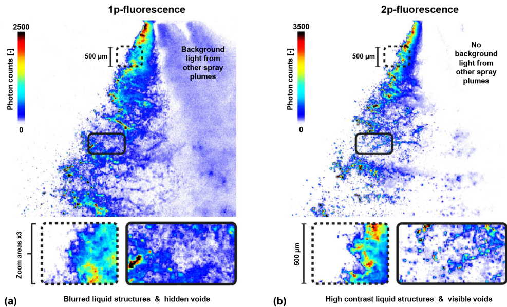
Fig. 9. Light sheet imaging comparison between 1p-LIF in (a) and 2p-LIF light sheet imaging in (b) for the 6 holes GDI spray injected at 200 bars liquid pressure and recorded at 200 \mu s. The two images have been recorded with the same camera system but corresponds to independent injection events. It is seen from the \times 3 zoom areas that 2p-LIF provides images with limited blur allowing the visibility of liquid structures which are not observable with the 1p-LIF scheme.
