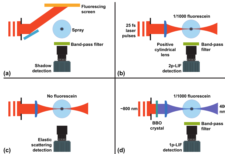
Fig. 5. Description of the optical arrangement for each detection configuration. The detection corresponding to shadowgraphy imaging, two-photon fluorescence, elastic light scattering and one-photon fluorescence are shown in (a), (b), (c) and (d) respectively.
