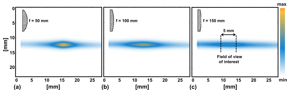
Fig. 2. Effect of the focal distance of a converging cylindrical lens on the generation of two-photon excitation fluorescence signal. Here, the focal distance corresponds to 50 mm, 100 mm and 150 mm in (a), (b) and (c) respectively. By using longer focal distances a more homogeneous two-photon fluorescence signal is generated.
