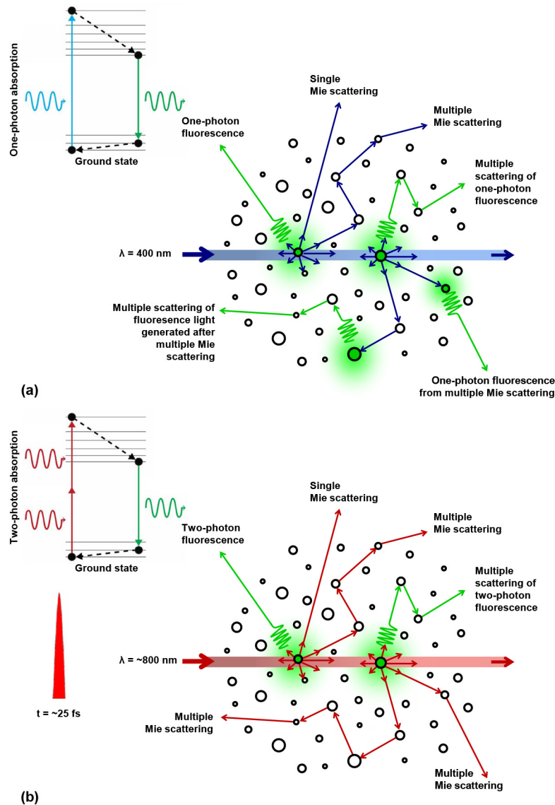
Fig. 3. Comparison between (a) single-photon and (b) two-photon excitation processes applied in a spray system consisting of a cloud of droplets. The fluorescence from two-photon excitation is only generated along the light sheet reducing a significant part of unwanted fluorescence outside of the light sheet.
