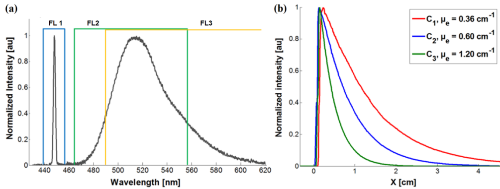
Fig. 2. (a): Emission spectra from yellow fluorescing highlighter's ink excited at 448 nm. The LIF signal is peaking at 517 nm. The Mie and LIF signals are filtered prior to detection, using two high-performance optical filters, FL1 and FL2 respectively. (b): Intensity decay of the laser sheet crossing a cuvette filled with dyed water for three different concentrations C_1 , C_2 and C_3 . These dye concentrations were successively tested in the spray. To avoid unwanted reflections effects from the cuvette walls, SLIPI LIF is performed here.
