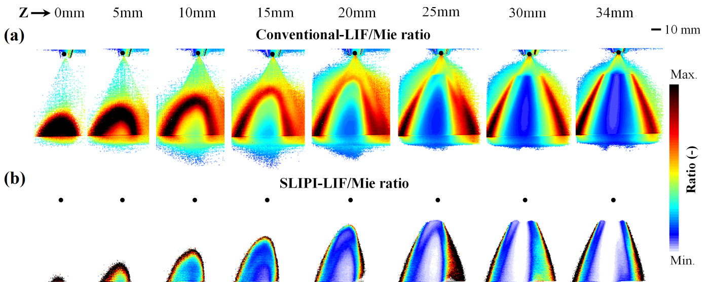
Fig. 3. (a) The averaged non-calibrated conventional LIF/Mie ratio images for positions 0 \leq Z \leq 34 mm is shown. Similarly, in (b), the averaged SLIPI LIF/Mie images are shown. By comparing (a) with (b), it is observed that the conventional-LIF/Mie ratio is not reliable since it produces ratio gradients in the spray regions which are not illuminated. For example, a non negligible ratio values are appearing from the region residing between the nozzle tip and the light sheet illumination.
