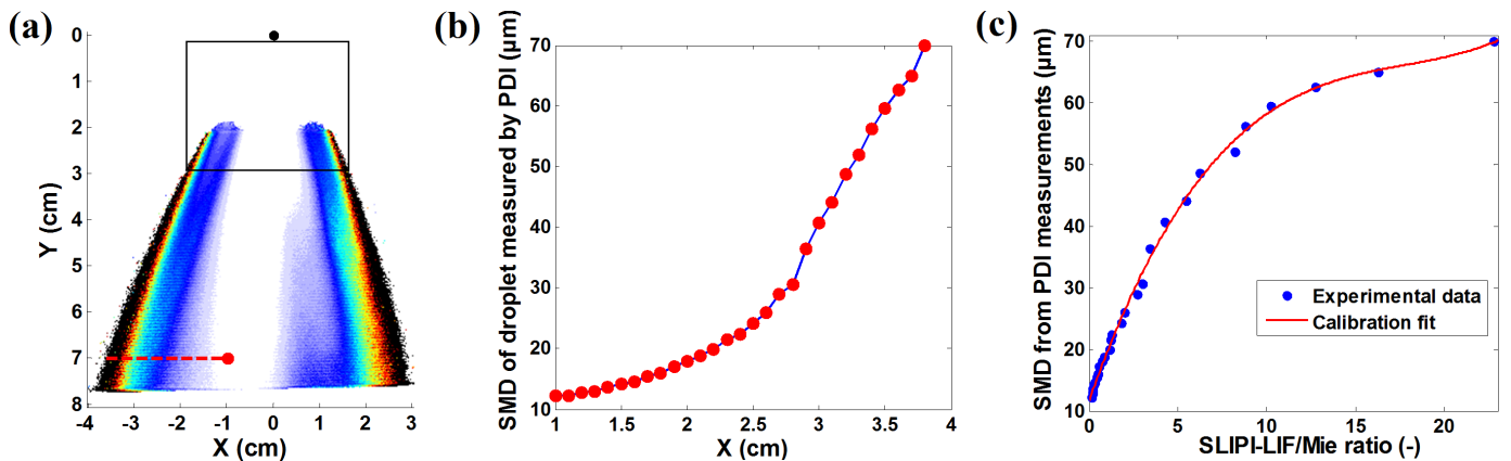
Fig. 4. (a) The SLIPI-LIF/Mie image showing the PDI calibration points located at Y = 7 cm and X = -1 to 3.7 cms. (b) Droplets SMD measured by PDI along the x-axis from one edge of the spray towards its center. For every millimeter measurement point the corresponding droplet size distribution is used to deduce the SMD in \mu\text{m} s. (c) The plot of the SMD values measured with PDI against the corresponding SLIPI-LIF/Mie ratio. A cubic fit is found to be best fit for converting the SLIPI ratio into droplet absolute SMD (see figures 6 and 7).
