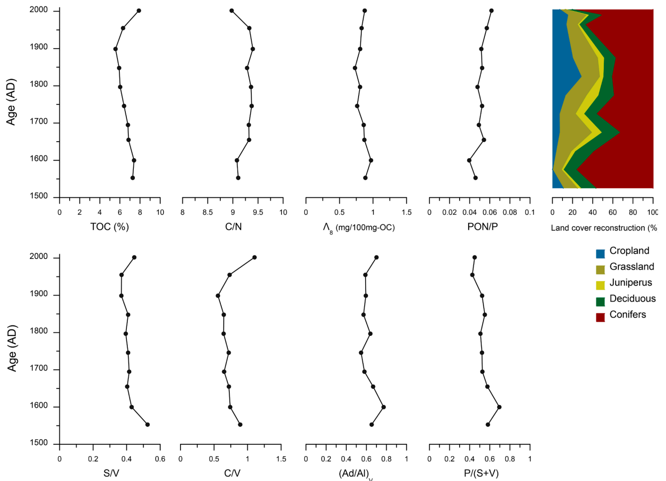
Figure 12 Total organic carbon content (TOC), carbon/nitrogen ratios (C/N), lignin data and land-cover reconstruction based on the pollen of the sediment record from Gåsfjärden. \Lambda_8 : sum of vanillyl, syringyl and cinnamyl phenols normalized to 100 mg organic carbon; PON/P: ratios of p -hydroxyacetophenone to total p -hydroxyl phenols; S/V: ratios of syringyl to vanillyl phenols; C/V: ratios of cinnamyl to vanillyl phenols; (Ad/Al) v : ratios of vanillic acid to vanillin; P/(S+V): ratios of p -hydroxyl to sum of vanillyl and syringyl phenols.
