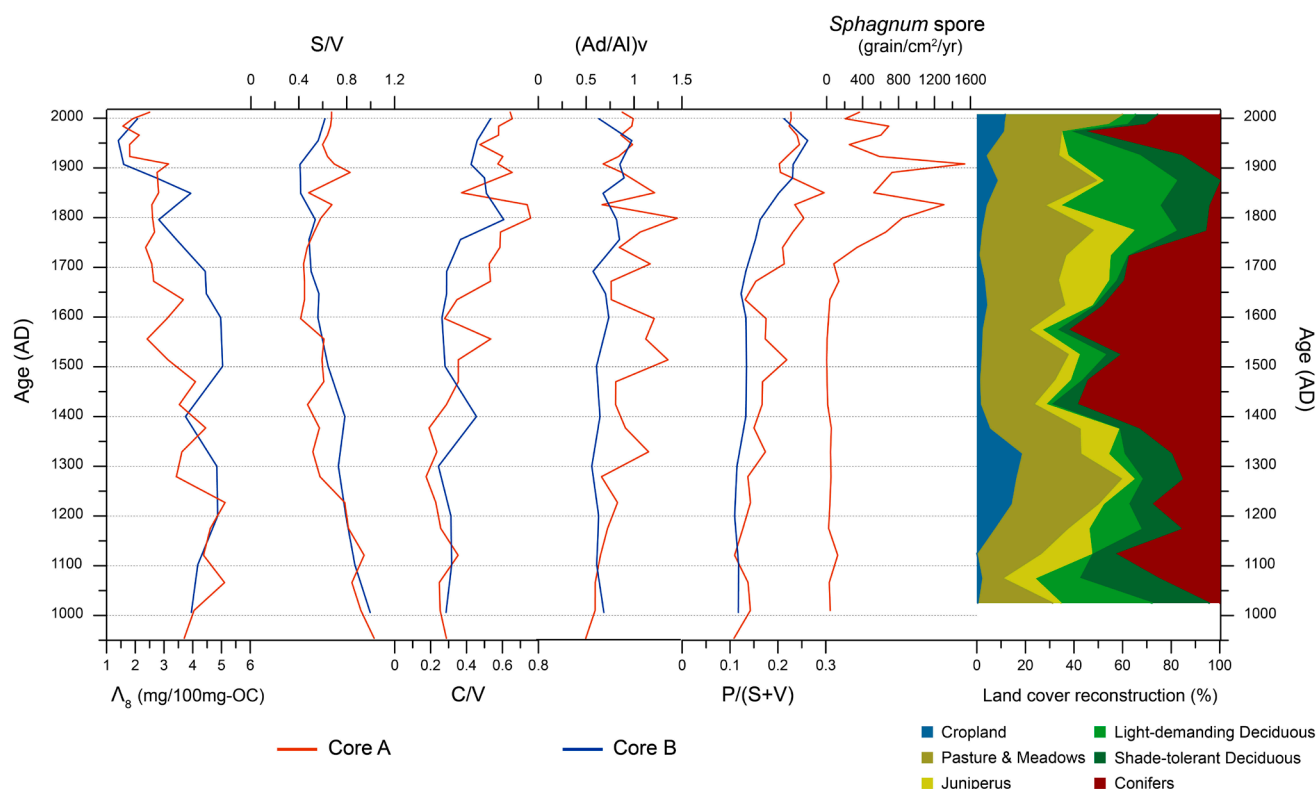
Figure 10 Lignin data from records A (red) and B (blue) together with Sphagnum spore accumulation rate and pollen-based land-cover reconstruction from Skottenesjön A. \Lambda_8 : sum of vanillyl, syringyl and cinnamyl phenols normalized to 100 mg organic carbon; S/V: ratios of syringyl to vanillyl phenols; C/V: ratios of cinnamyl to vanillyl phenols; (Ad/Al) v : ratios of vanillic acid to vanillin; P/(S+V): ratios of p -hydroxyl to sum of vanillyl and syringyl phenols. Land-cover reconstruction is based on Yang et al. (2020).
