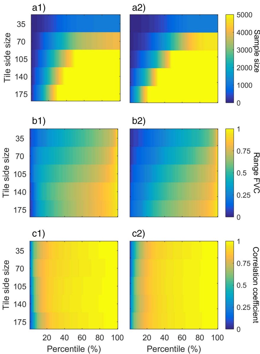
Fig. 4. Influence of tile size (y-axis) on the percentiles of the time series (x-axis) of the parameters influencing the triangular shape. a) Number of points including in the triangle (N); b) range in fraction of vegetation cover (FVC); and c) correlation coefficient of the dry edge slope (r) for 1) the Dahra and, 2) the Nalohou field sites. The percentiles on the x-axis gives an indication of the fraction of the time-series for a given tile size having a range smaller than the value shown by the colour.
