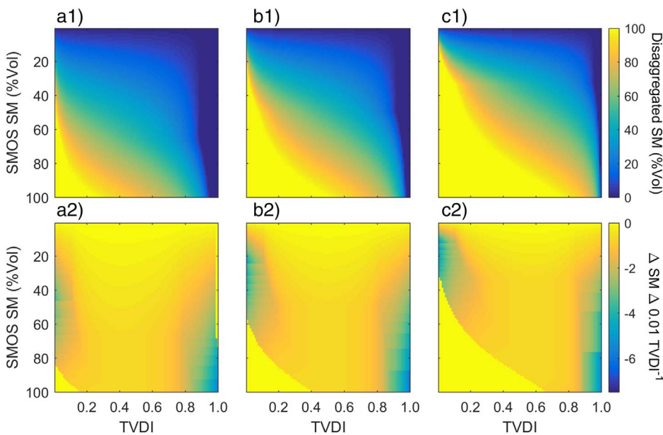
Fig. 8. Sensitivity of disaggregated SMOS soil moisture (SM; %Vol) to changes in TVDI. Average TVDI in Eq. 8 was set to a) 0.25, b) 0.50 and c) 0.75. First row (1) shows the actual disaggregated SM for each original SMOS SM -TVDI case and second row (2) shows the changes in disaggregated SM for each 0.01 error in TVDI for each SM-TVDI case.
