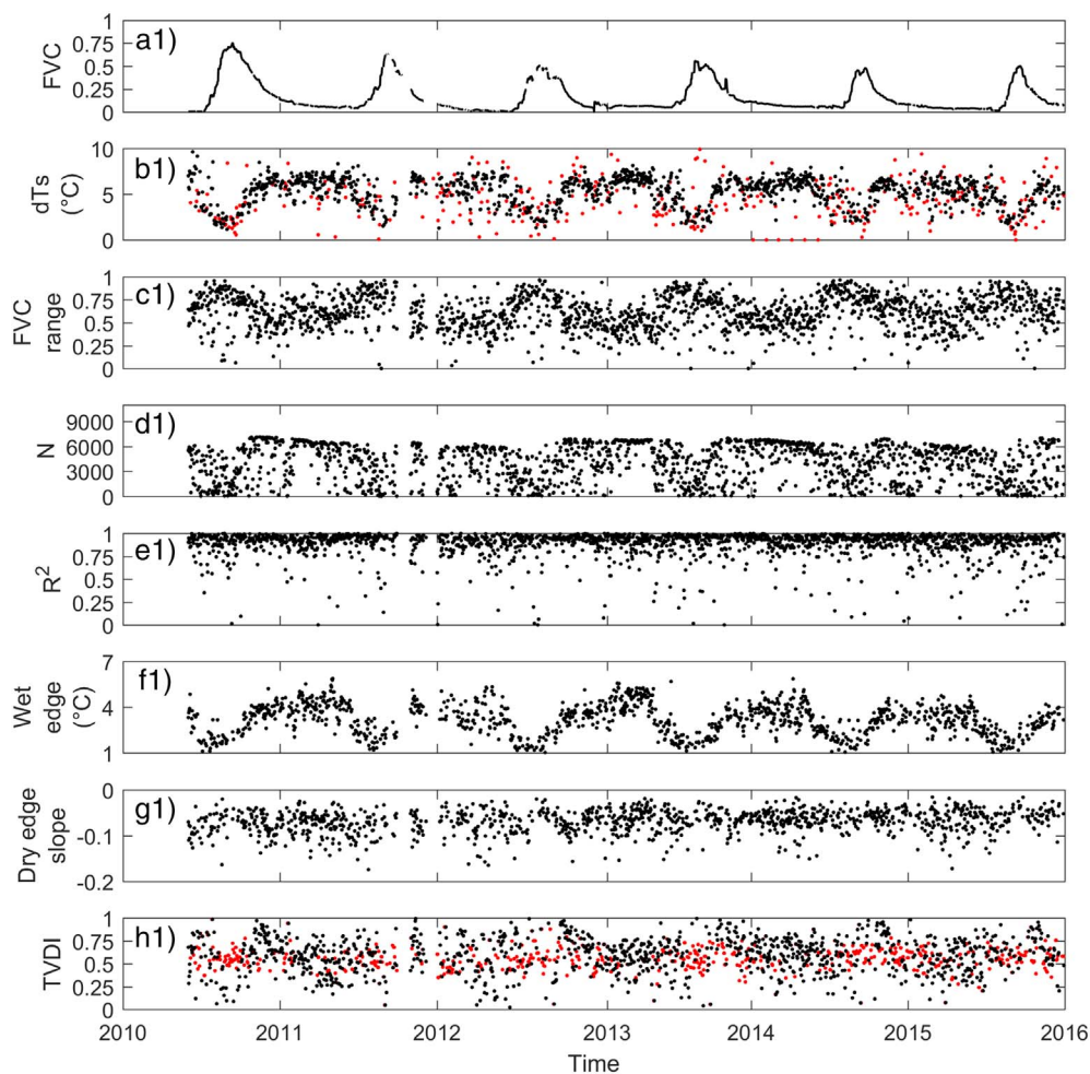
Fig. 6. Time series of the input parameters, extracts from the TVDI calculation tiles, and final TVDI estimates for (1) Dahra and (2) Nalohou: (a.) fraction of vegetation cover (FVC); (b) unfiltered (red) and filtered (black) morning rise temperature ( dT_s ); (c) range of FVC in the TVDI tiles; (d) total number of points included in the triangle ( N ); (e) coefficient of determination ( R^2 ) for the dry edge fit; (f) wet edge; and (g) dry edge slope. Included are also (h) filtered (black) and gap-filled (red) TVDI estimates (black). (For interpretation of the references to colour in this figure legend, the reader is referred to the web version of this article.)
