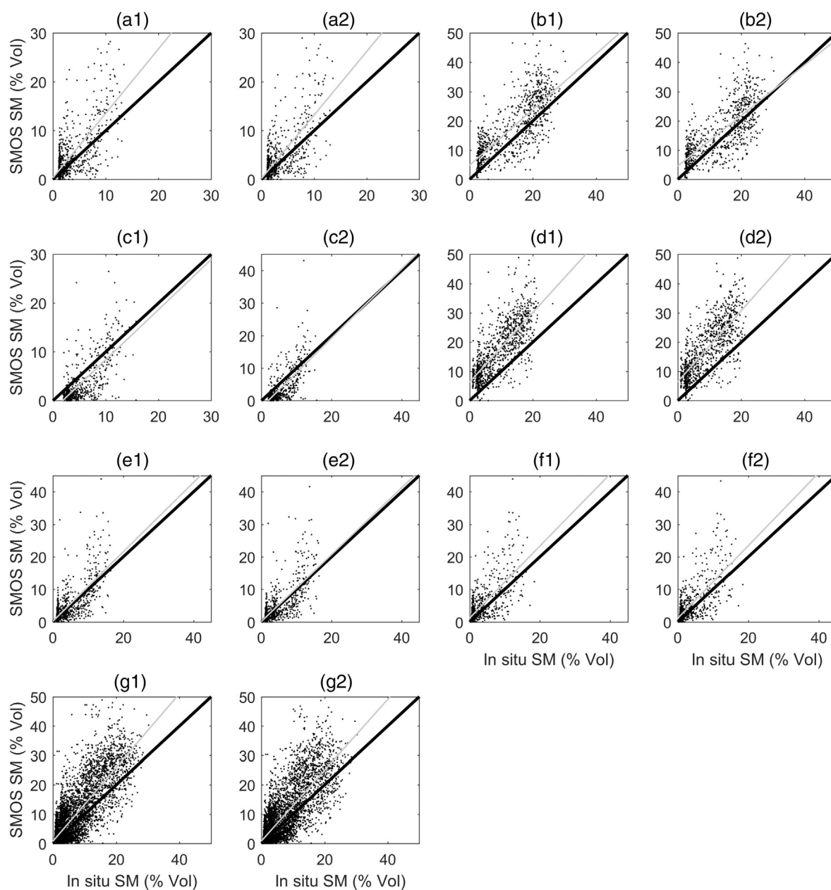
Fig. 10. Relationship between in situ and both original (1) and disaggregated (2) Soil Moisture and Ocean Salinity (SMOS) soil moisture (SM; %Vol) for the pixels used in the evaluation of the disaggregation methodology. The subplots are: a) Banizoumbou; b) Belefontougou; c) Dahra; d) Nalohou; e) Tondikiboro; f) Wankama; and g) all sites combined. The grey line is the ordinary least square linear regression and the black line is the one-to-one ratio. Statistics of the slopes are given in Table 1. The location of the sites can be seen in Fig. 2.
