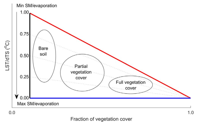
Fig. 1. Conceptual triangle space with the land surface temperature (LST) or morning rise temperature (dTS) on the y-axis and Fraction of Vegetation Cover (FVC) on the x-axis. The blue line is the wet edge (TVDI = 0.00) and the red line is the dry edge (TVDI = 1.00). The grey dotted lines are TVDI examples of 0.25, 0.50, and 0.75. The figure is adapted from Peng et al. (2017). (For interpretation of the references to colour in this figure legend, the reader is referred to the web version of this article.)
