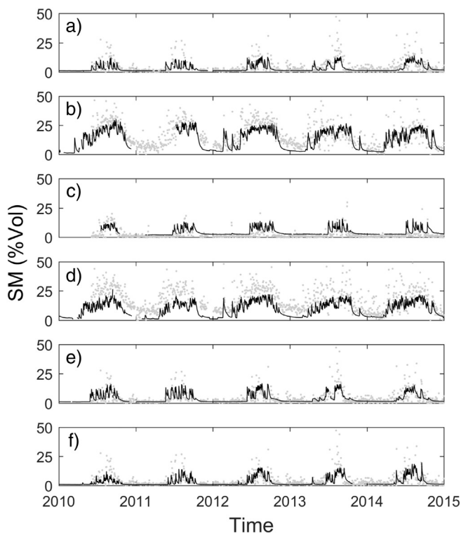
Fig. 9. Time series of in situ measured soil moisture (SM (%Vol)) (thin black line) and Soil moisture and Ocean Salinity (SMOS) SM (grey dots) for: a) Banizoumbou; b) Belefoungou; c) Dahr; d) Nalohou; e) Tondikiboro; and f) Wankama. The location of the different sites is shown in Fig. 2.
