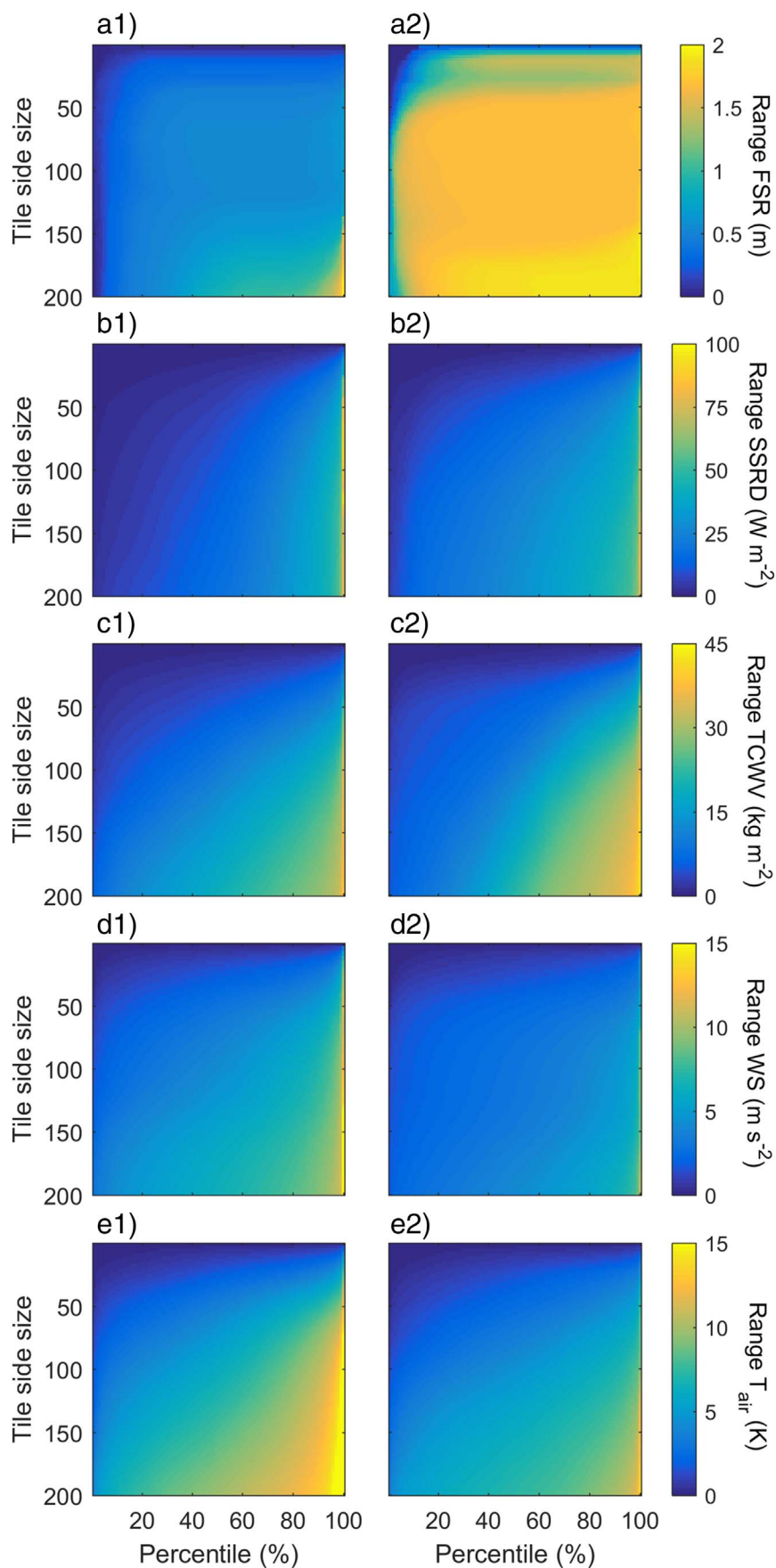
Fig. 3. Dynamic range in surface properties and atmospheric forcing influencing the homogeneity of available energy within the triangular space. Influence of tile size (y-axis) on the percentiles of the time series (x-axis) of the dynamic range in daily averaged a) forecast surface roughness (FSR) (m); b), surface solar radiation downwards (SSRD) ( \text{W m}^{-2} ); c) total column water vapour (TCWV) ( \text{kg m}^{-2} ); d) wind speed at 100 m height (WS) ( \text{m s}^{-1} ); and e) air temperature at the 975 hPa level ( T_{\text{air}} ) (K) for 1) the Dahra and 2) the Nalohou field sites. The percentiles on the x-axis gives an indication of the fraction of the time series for a given tile size having a dynamic range smaller than the value shown by the colour. For the z-axis, dark blue indicates high homogeneity ( i.e. small dynamic range) in surface properties or atmospheric forcing, whereas yellow indicates low homogeneity. (For interpretation of the references to colour in this figure legend, the reader is referred to the web version of this article.)
