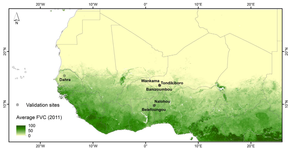
Fig. 2. Study area with the location of the in situ validation sites. The averaged fraction of vegetation cover (FVC) for year 2011 is used as background to illustrate the important north-south gradient in vegetation cover.
