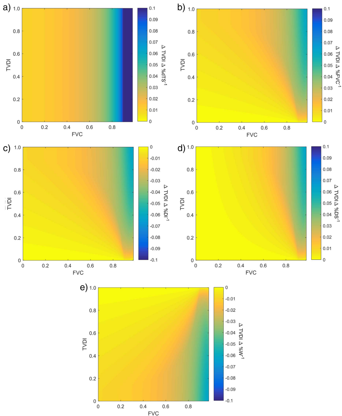
Fig. 7. Sensitivity of TVDI to input data and equation parameters: a) morning rise temperature (dTS; °C); b) fraction of vegetation cover (FVC); c) dry edge intercept (DI); d) dry edge slope (DS); and e) wet edge (W). The % for the temperatures (dTS, DI, and W) and the FVC is a % change in relation to the range of the triangle. During the analysis we changed one parameter at the time and the rest remained stable.
