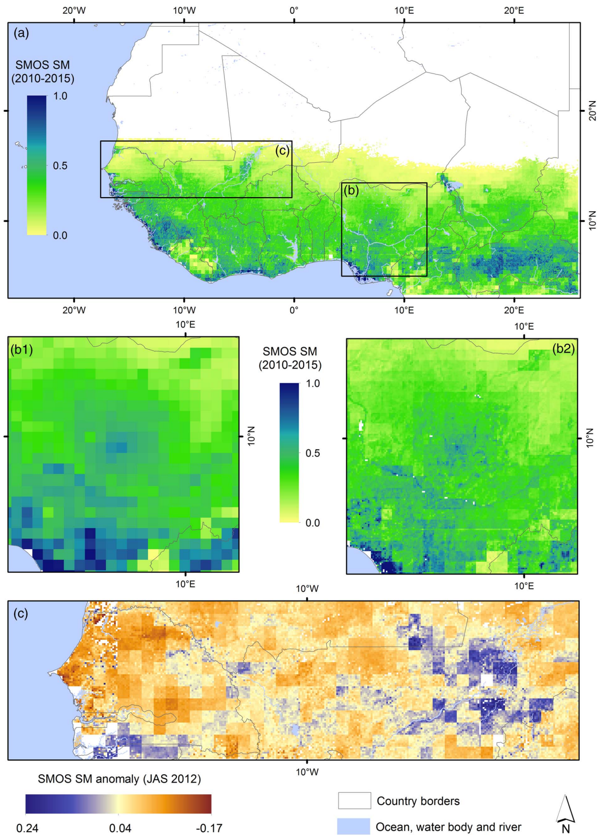
Fig. 11. Average soil moisture (SM) 2010–2015 derived from the disaggregated SMOS product over West Africa (a). Main river networks were not visible in the original (non-disaggregated) products (b1), whereas they became apparent after disaggregation (b2). SM extremes (flood and drought) were also captured for the test case of JAS 2012 (c). Filtered and no data are represented in white. The blocky structure observed in the disaggregated products are caused by the original SMOS pixel resolution.
