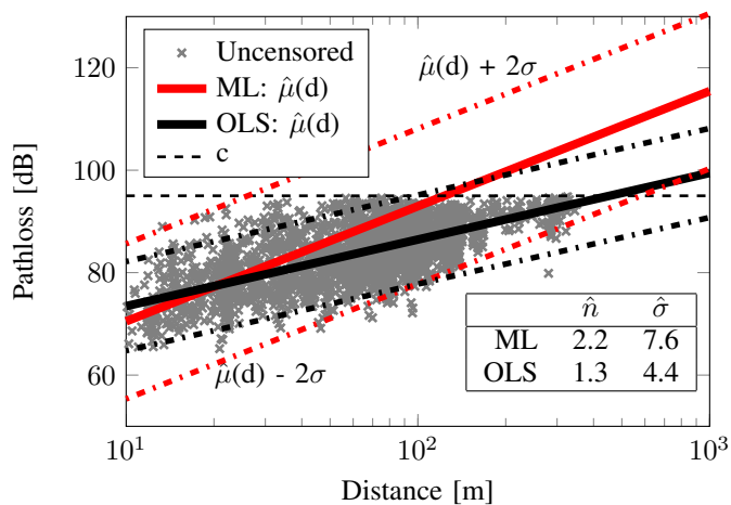
Fig. 2. Pathloss estimation of censored measurement data, using ML and OLS estimation. The estimated standard error for the ML estimates are SE(\hat{P}L(d_0)) = 0.72 dB, SE(\hat{n}) = 0.04 and SE(\hat{\sigma}^2) = 1.6 .
