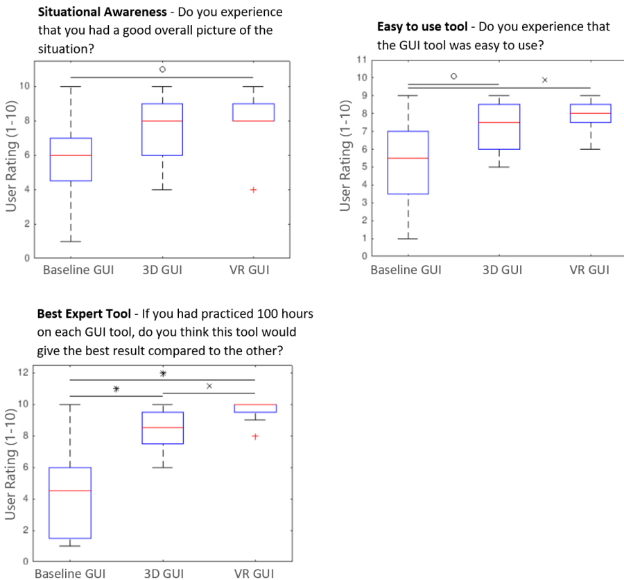
Figure IV.10: The evaluation score for Situational Awareness , Easy to Use and Expert Tool have been improved for the users of the 3D GUI , and improved even more for the users of the VR GUI . (o), (x) and (*) denote comparisons with p < 0.05 , p < 0.01 and p < 0.001 respectively.
