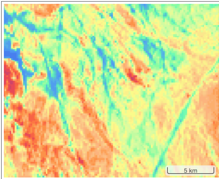
Figure I.5: The figure shows a publicly available magnetic field map. Each pixel corresponds to a square with a size of 185m×185m.
