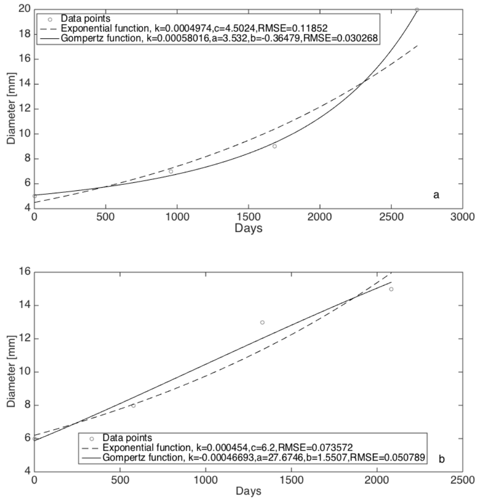
Figure 3. Example of tumour growth curves described by an exponential and a Gompertz function, respectively (a,b). In (b) the Gompertz function is modelled in the late decelerating growth rate phase.
