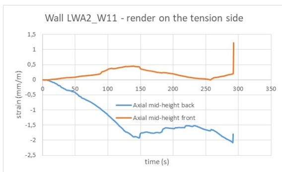
Figure LWA2_W12_3 Axial strains at mid-height vs. time – front (tension) and back (compression) side.
