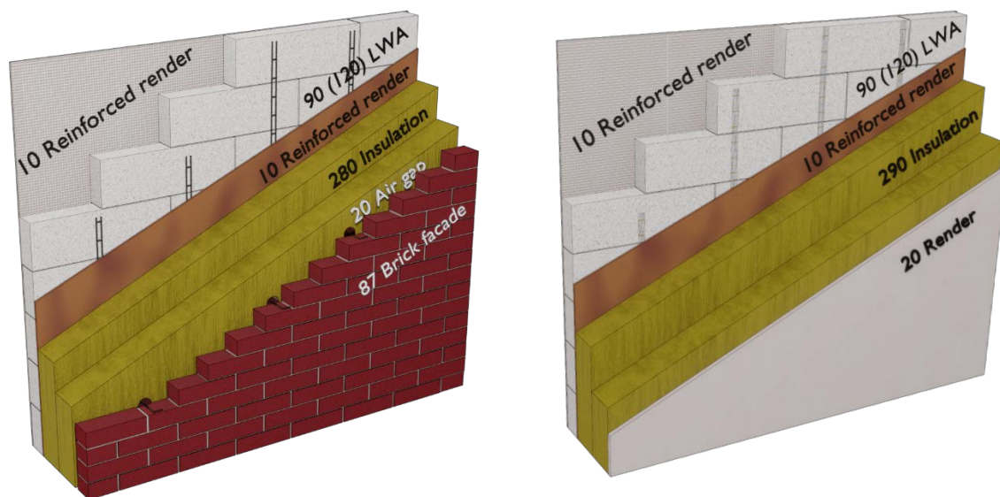
Figure 1.1 Exterior walls with improved thermal performance.
