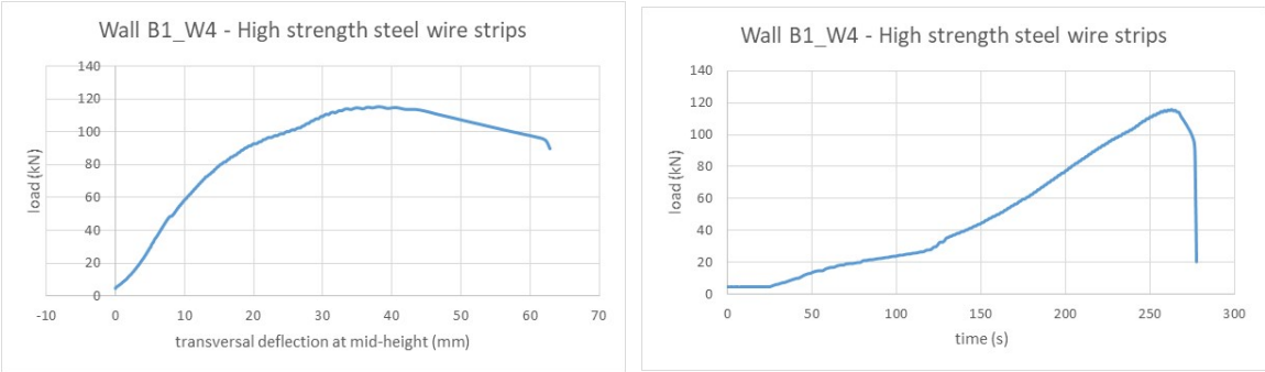
Figure B1_W4_2 Load vs. transversal deflection at mid-height (left); load vs time (right).
