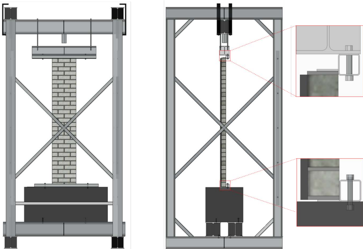
Figure 2.10 Rig for testing walls in bending and vertical axial loading.
