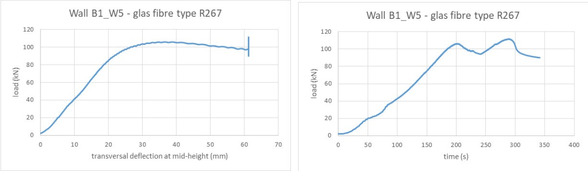
Figure B1_W5_1 Load vs. transversal deflection at mid-height (left); load vs. time (right).
