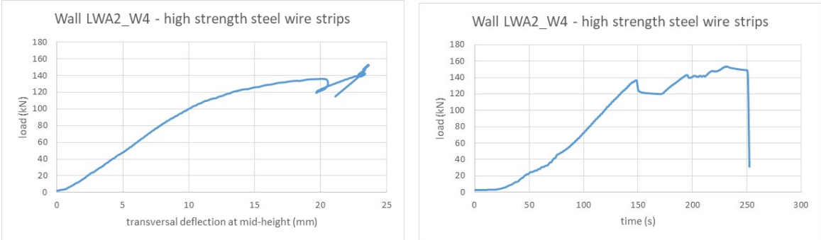
Figure LWA2_W4_2 Load vs. transversal deflection at mid-height (left); Load vs. time (right)
