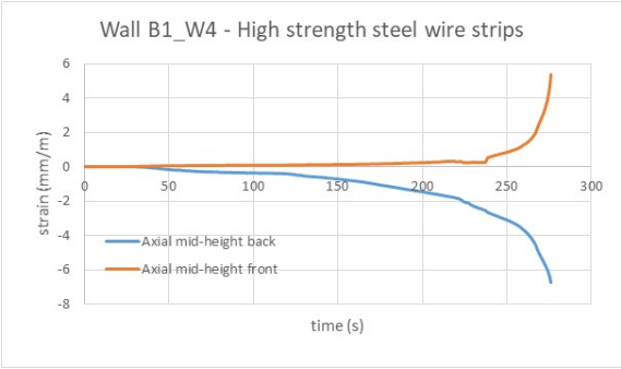
Figure B1_W4_3 Axial strains at mid-height vs. time – front (tension) and back (compression) side.
