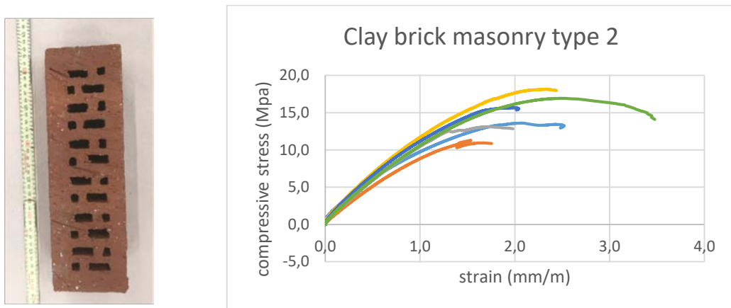
Figure 2.2 Clay brick masonry type 2. Perforated bricks (left); stress – strain relationship (right).
