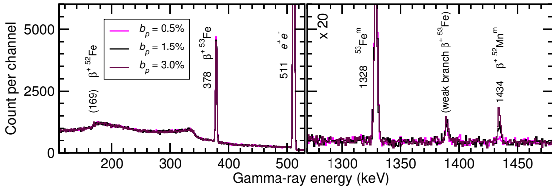
FIGURE 4. Simulated \gamma -ray energy spectra in prompt ( \Delta t = 300 ns) coincidence with a 0.1-3.0-MeV particle detected in the central 'deposition DSSSD' assuming different proton-decay branching ratios, b_p . Energy labels are in keV.
