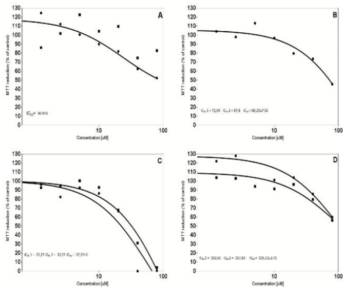
Figure 1. Dose response curves and IC_{50} values of isolated saponin obtained by treatment of JIMT-1 breast cancer cells. The dose response was evaluated with a MTT assay after 72 hours of incubation with each compound. Each curve shows an independent experiment ( n=6 ). A. (1) Oleanolic acid, B. (2) Methyl oleanate, C. (3) Hederagenine, D. (4) Phytolaccagenic acid
