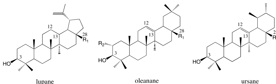
Figure 9. Molecule structures of lupane, oleanane, and ursane
