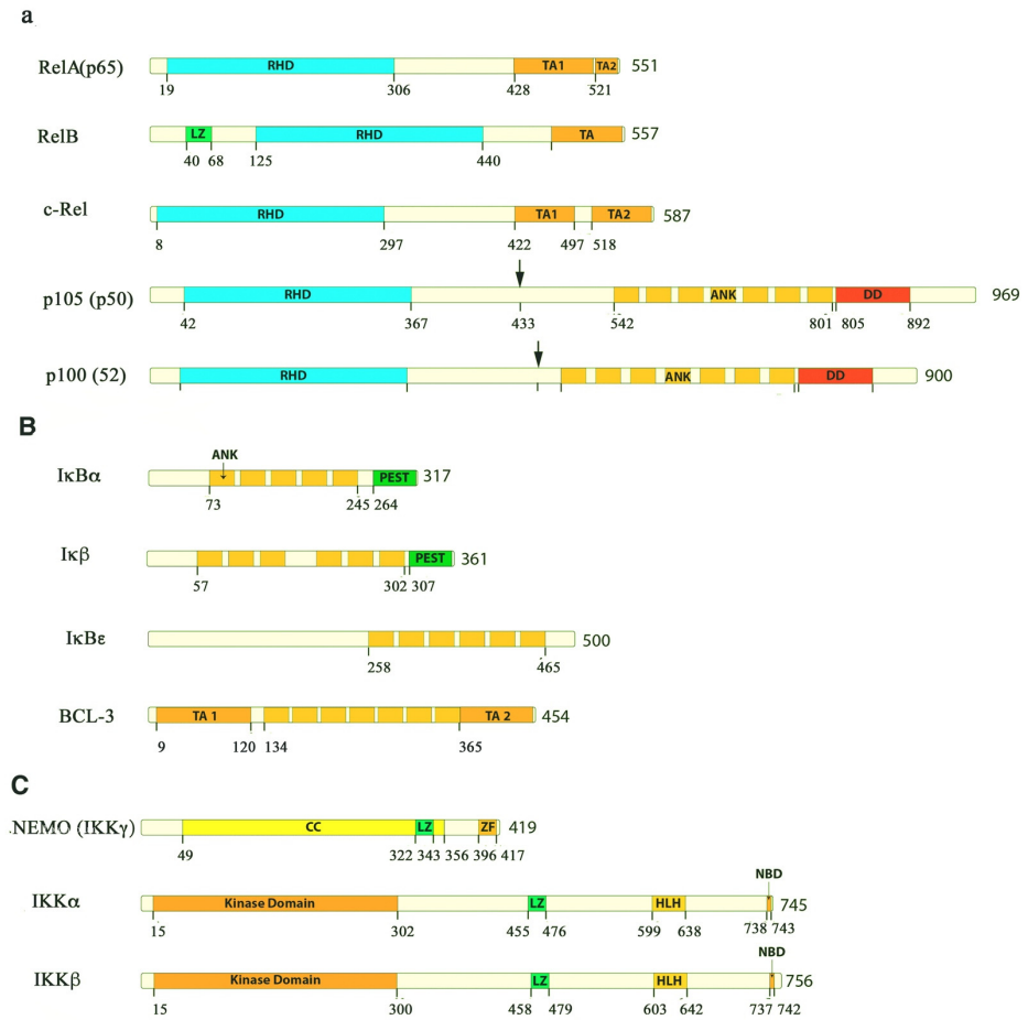
Figure 12. Members of the A) NF- \kappa B (Rel family), B) I \kappa B family and C) IKK complex. The numbers of amino acids in each the human protein is indicated on the right . All members of NF- \kappa B may share a rel homology domain (RHD) which is required for their dimerisation.
