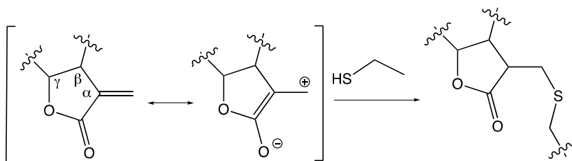
Figure 4. A Michael addition reaction of a thiol to the \alpha -methylene- \gamma -lactone moiety of a \alpha MyL-STL.
