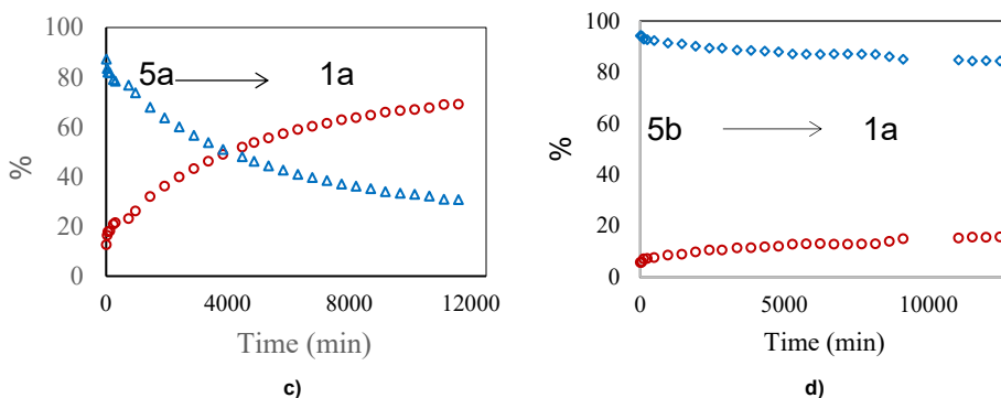
Figure 27. The stability of the thiol adducts c) thiol-damsin adduct isomer 5a and d) thiol-damsin adduct isomer 5b
