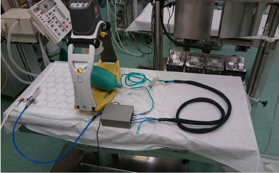
Our ventilator research prototype (gray box with tubing) together with the commercially available LUCAS chest compression device, developed at Igelösa.
