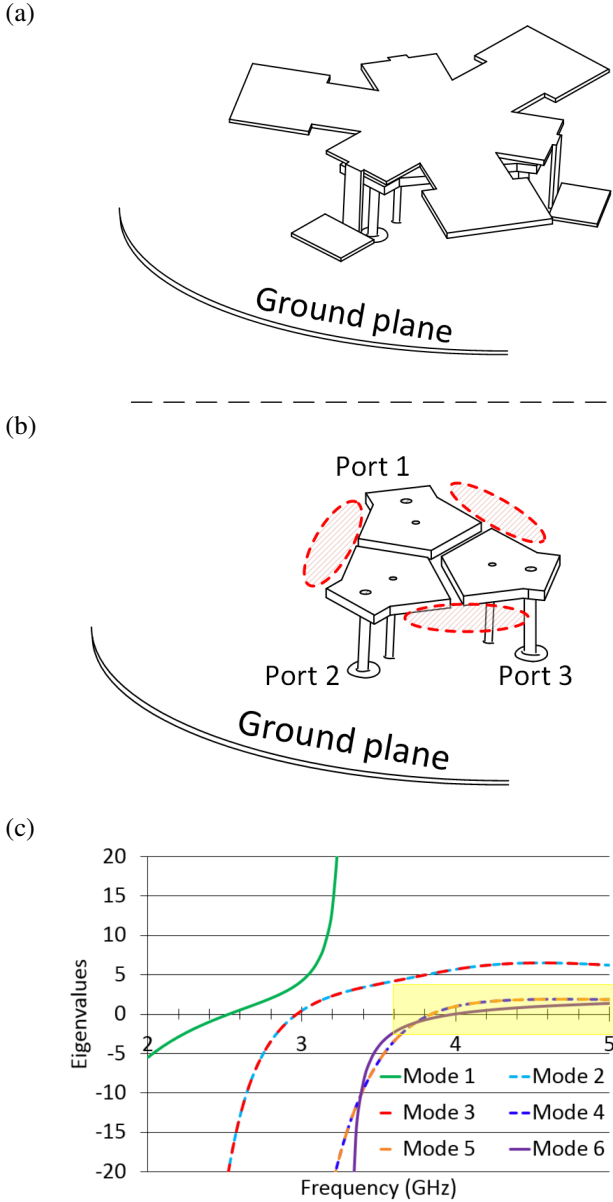
Fig. 2. Broadside tri-modal patch antenna in [24]: (a) overall structure; (b) capacitive loading plates with shorting pins; (c) eigenvalues (first six modes).
