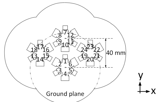
Fig. 13. Geometry of four elements co-designed two broadside tri-modal patch MIMO array.
