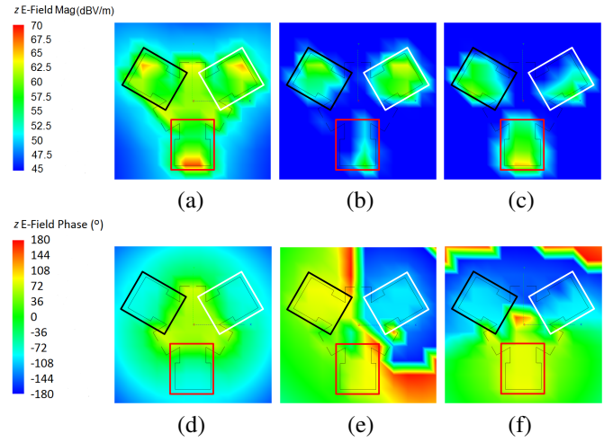
Fig. 4. The z -directed characteristic E-fields at 0.2 mm below the top snowflake patch in [24]: amplitude distribution of the first three modes at 5.5 GHz correspond to (a)–(c); phase distribution of the first three modes at 5.5 GHz correspond to (d)–(f).
