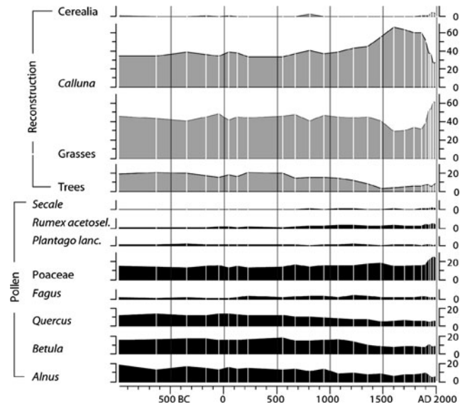
Fig. 12 Kragssø. LRA-reconstruction of the cover of cereals, heather, grasses and trees through the last 3,000 years. A selection of frequencies (percentage of terrestrial pollen) of the more important pollen types is also shown
