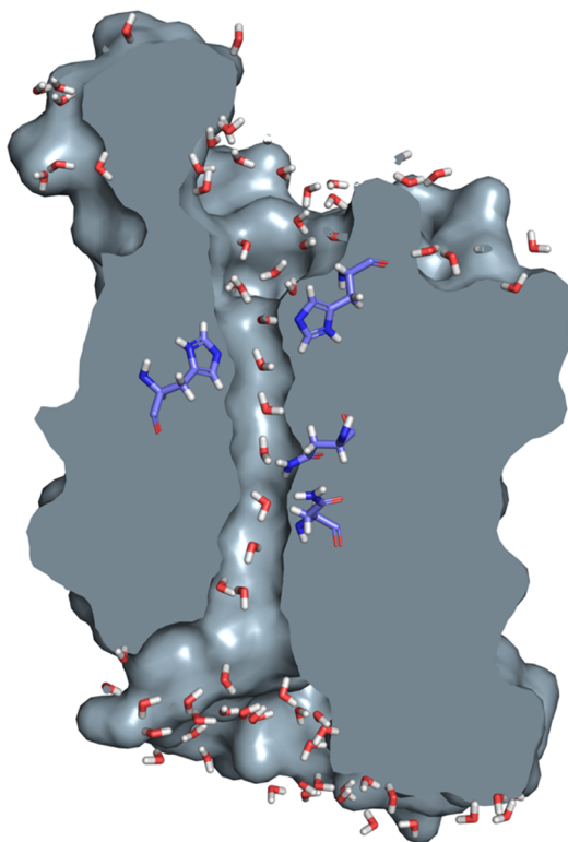
Figure 2. A surface representation of the monomeric structure of AtTIP2;1 cut open to show the bi-directional orientation of the water molecules in the pore. An energy minimization was done on the water molecules with the protein fixed in NAMD [Philips et al. , 2005]. The hydrogens of the water molecules in the pore point away from the center of the protein. For simplicity, only the two asparagines in the NPA region (one from each half helix) and the two histidines (at H2 P and LC P positions) in the ar/R filter are shown. This structure was adapted from the X-ray crystal structure (PDB ID 5I32) of AtTIP2;1 [Kirscht et al. , 2016a]. Molecular dynamics simulations were done by Yonathan Sonntag.
