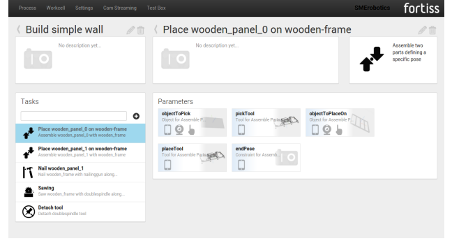
Figure 6 Woodworking process parsed from BTL and visualized in the intuitive instruction GUI. Parameters for each task can be modified before execution.
