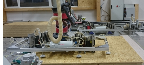
(b) Nailing of panels to wall structure.
