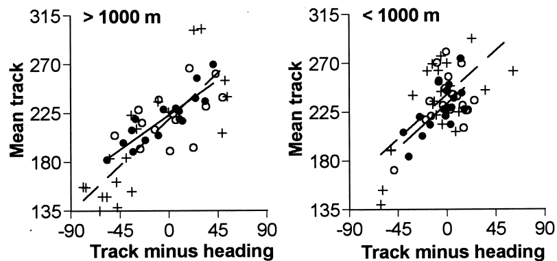
Fig. 9. Nightly mean track direction in relation to track direction minus heading direction of birds flying above and below 1000 \text{ m} ASL, respectively. Nights with intense migration are marked with a dot, intermediate intensity with an open circle and low intensity with a cross. The slope of the regression line is a measure of the magnitude of drift or compensation for drift ( b = 1 means full drift and b = 0 complete compensation) (Alerstam 1976a) (Intense migration: < 1000 \text{ m ASL} , b = 0.91 \pm 0.16 ( 95\% confidence interval), > 1000 \text{ m ASL} , b = 0.71 \pm 0.07 , solid lines; low intensity migration: < 1000 \text{ m ASL} , b = 0.90 \pm 0.15 , > 1000 \text{ m ASL} , b = 0.92 \pm 0.12 , broken lines) (see text for more statistics).
