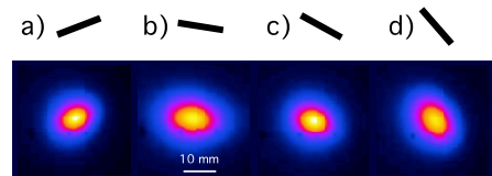
FIG. 3 (color online). Representative data showing the variation of electron beam profile with laser polarization at n_e = 2.2 \times 10^{19} \text{ cm}^{-3} with a pulse duration of 68 fs. The black line indicates the laser polarization angle \pm 5^\circ . (a) -20^\circ , (b) 10^\circ , (c) 30^\circ , and (d) 50^\circ .
