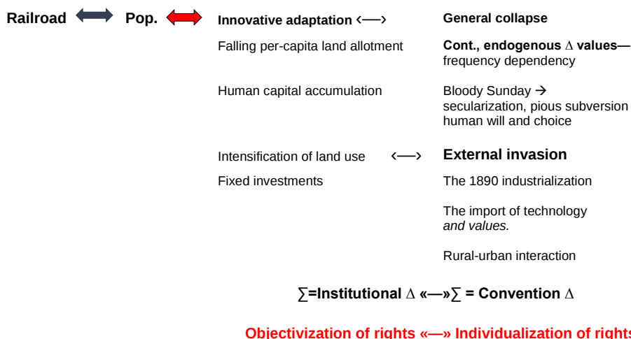
Figure 3-5 Back to Theory: The Regulationist–Institutionalist Summarizing Loop
