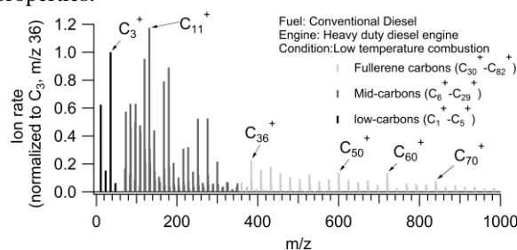
Figure 1. SP-AMS refractory mass spectrum of soot from low temperature diesel combustion. The spectrum has been normalized to the C_3^+ intensity.
