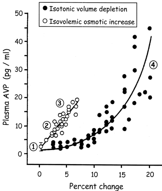
Figure 4: Percentual increase in plasma osmolality and percentual decrease in blood volume as stimuli for progressive AVP secretion in rat. Levels 1 and 2 correspond to moderate osmotic stimulation occurring in usual life. Level 3 corresponds to mild dehydration. Higher values of plasma AVP (level 4) usually occurs after severe dehydration or reduced extracellular fluid volume. Changes in blood volume were achieved by injection of intraperitoneal polyethylene glycol, leading to reductions in blood volume without altering plasma osmolality. Reprinted by permission from Oxford University Press: Cardiovascular research, Bankir, L., Antidiuretic action of vasopressin: quantitative aspects and interaction between V1a and V2 receptor-mediated effects. 2001. 51: p. 372-90 Copyright © 2001.
