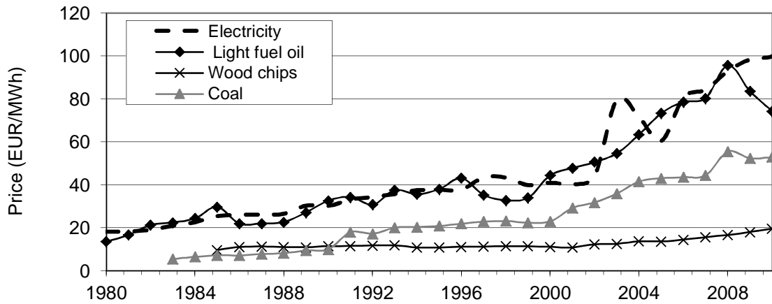
Figure 3: Nominal fuel and electricity prices, including taxes, paid by Swedish DH producers in 1980-2010. The fuel prices after 2004 refer to fuels used in heat production only, since fuels used in CHP production were taxed differently after 2004 (SEA, 2009; SEA, 2013).
