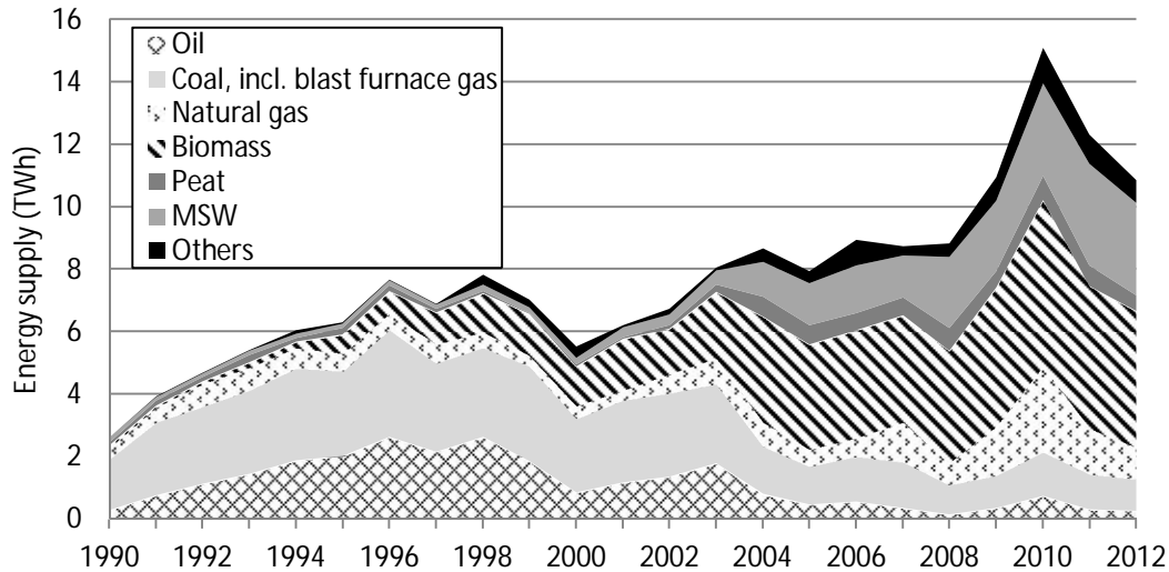
Figure 4: Energy supply for electricity production in CHP plants in Swedish DH systems in 1990-2012 (SCB, 2014).
