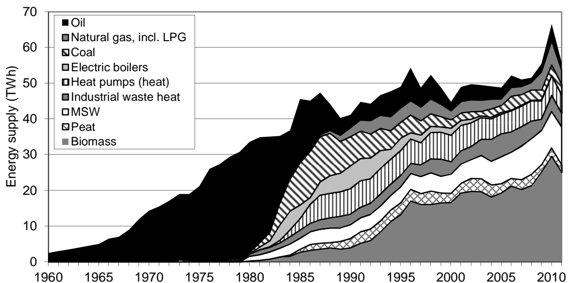
Figure 2: Energy supply in Swedish DH production, 1960-2011. The energy supply that can be attributed to electricity production in CHP plants is not included. 1960-1969: approximations from SDHA (2001); 1970-2010 from SEA (2012); 2011 from SEA (2013). Sharp annual variations are caused by variations in the outdoor temperature between years. For example, the winter of 2010 was unusually cold in Sweden.
