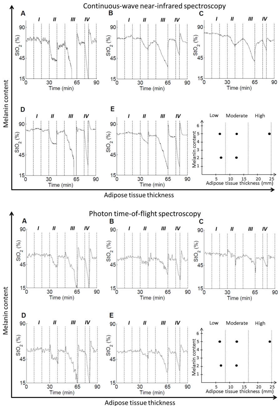
Figure 27. Diagrams showing influence of skin content of melanin and adipose tissue thickness in five individual recordings of \text{StO}_2 with continuous-wave near infrared spectroscopy (upper) and photon time-of-flight spectroscopy (lower) techniques under various experimentally induced regional physiological conditions (I-IV). Subject characteristics, corresponding to curves A-E, are shown in the lower right part of each diagram. From Paper II.
