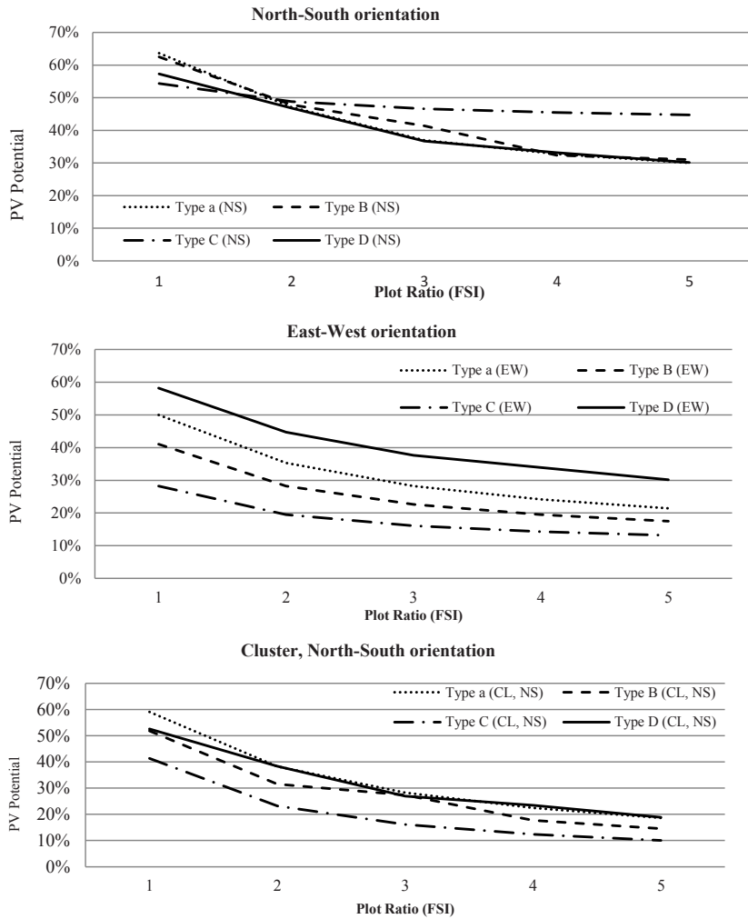
Fig. 4. PV potential of the blocks
