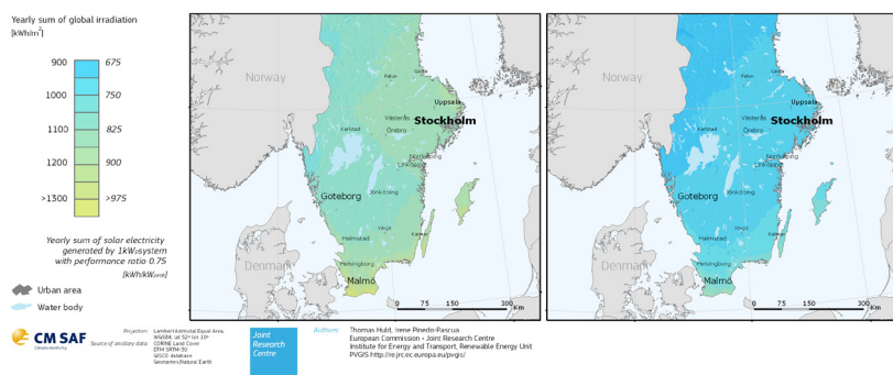
Figure 1.5 Irradiation on an optimal inclination (left) and on a horizontal plane (right) in southern Sweden (PVGIS, 2006)
