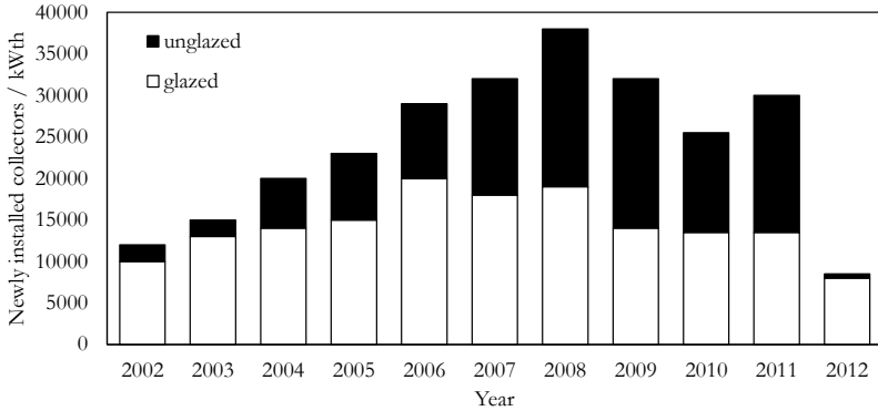
Figure 1.10 Development of ST market in Sweden (IEA, 2014)
