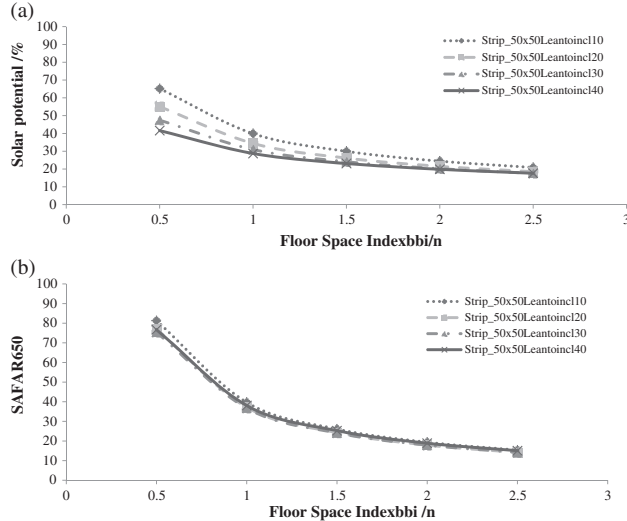
Figure 4. Solar potential as the percentage of building envelope which receives an amount of solar radiation greater than or equal 650 kWh/m 2 a (after Compagnon (2004)). Solar potential as the percentage of the building envelope which receives an amount of solar radiation greater than or equal 650 kWh/m 2 a related to the floor area (SAFAR 650 ).
