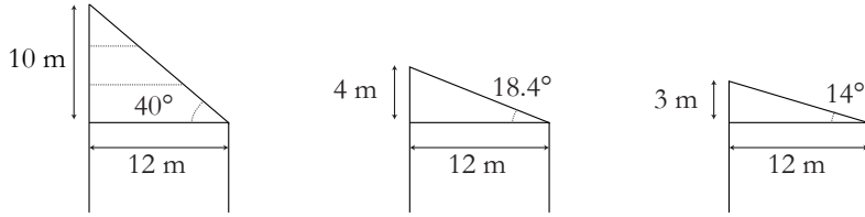
Figure 6.6 Consequences of roof types on building height
