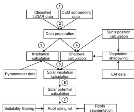
Figure 1. Methodology to produce a solar map [11]
