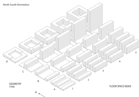
Fig. 1. Overview of geometry types in North-South orientation
