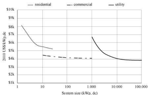
Figure 5. Residential, commercial, and utility scale PV system prices (installed) [13]
