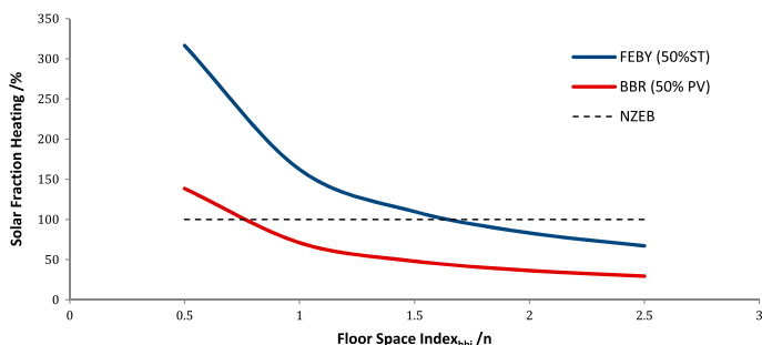
Figure 11. Load matching for heating demand (generalised).
