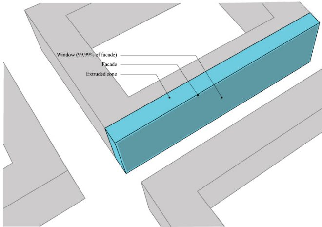
Figure 2. Construction of EnergyPlus simulation.
