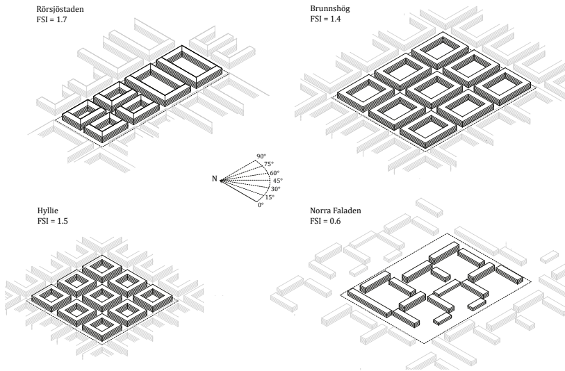
Figure 6.1 The four simulated city blocks and their actual FSI
