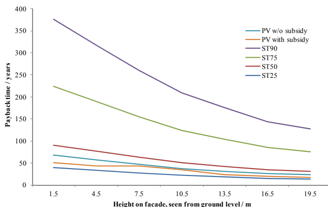
Figure 8. Payback time as a function of height.
