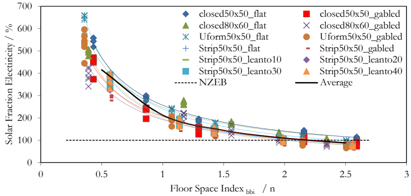
Figure 6.5 FEBY / BBR load matching for electricity demand
