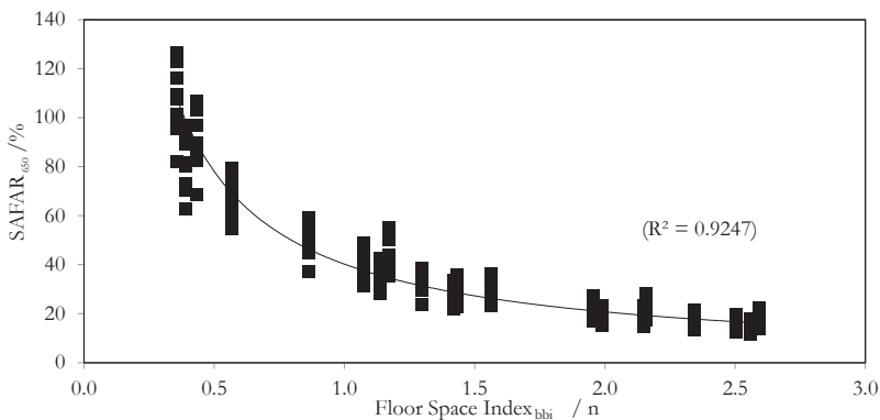
Figure 6.4 SAFAR 650 for all design options (averaged for all orientations)
