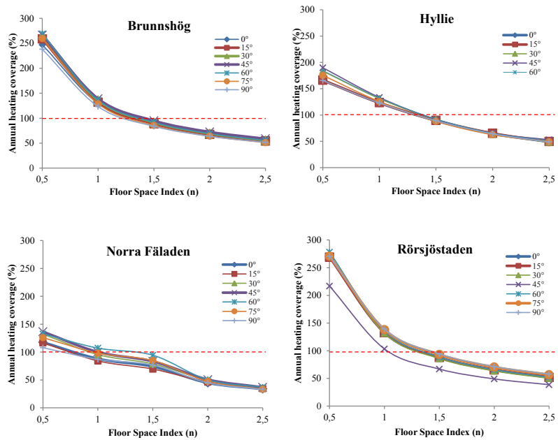
Figure 6: Annual heating coverage at different densities
