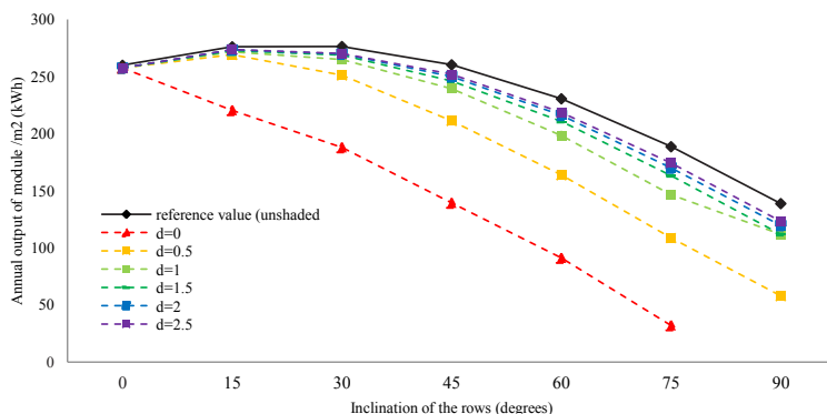
Figure 4. Output of the reference module and the shaded module in Miami.
