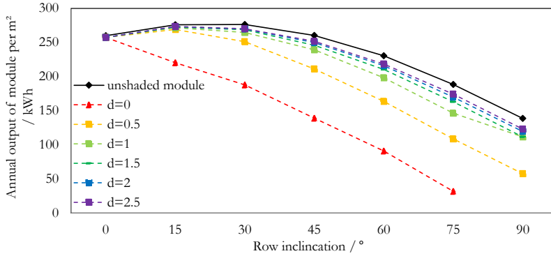
Figure 4.4 Output of the reference module and the shaded module in Miami
