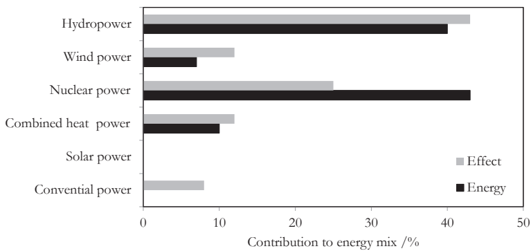
Figure 1.7 Distribution of installed effect and provided annual energy for different energy sources in 2013 in Sweden
