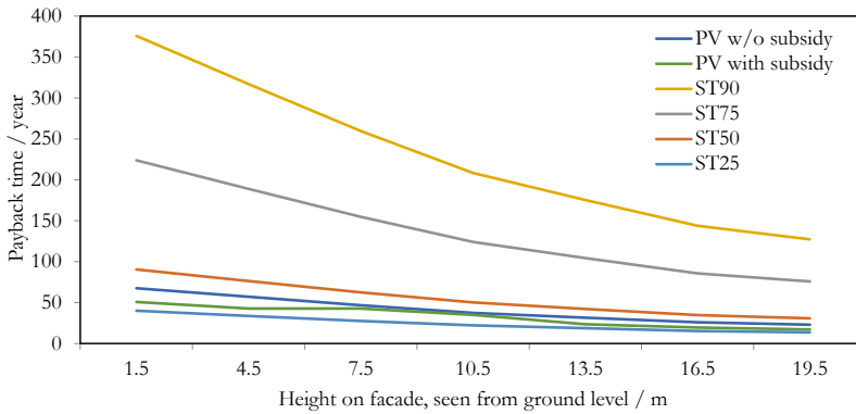
Figure 5.4 Payback time as a function of height
