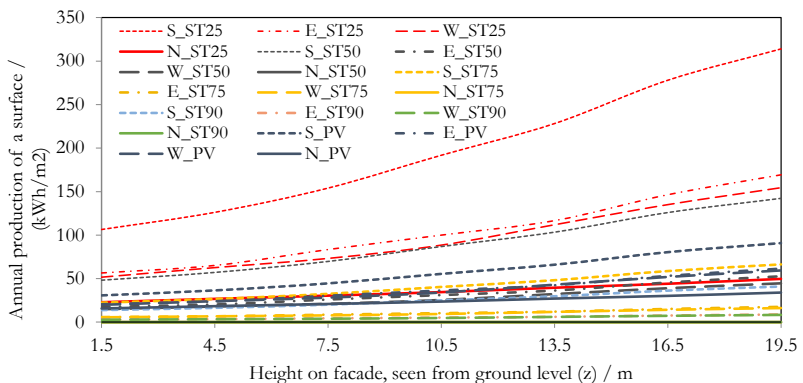
Figure 5.3 The annual energy production as a function of height from ground. The value after ST and PV corresponds to the system temperature (25°, 50°, 75°, 90°C)
