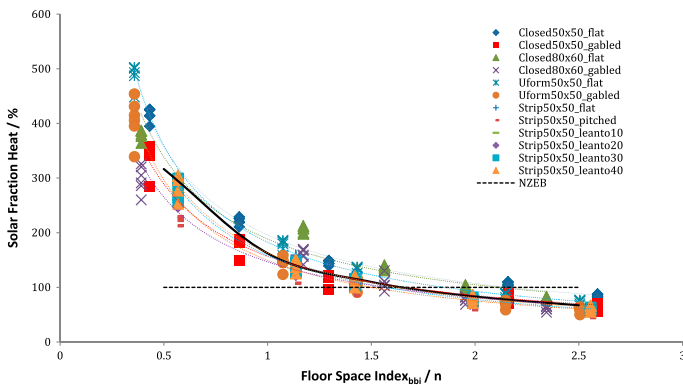
Figure 8. FEBY load matching for heating demand.
