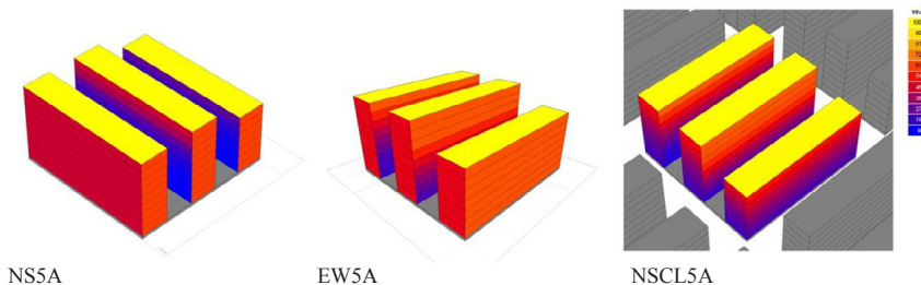
Fig. 3. Graphical output of annual solar insolation in Ecotect
