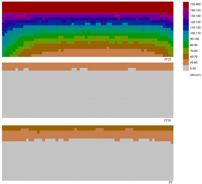
Figure 5.5 Annual production of ST 25°C, ST 50°C and PV on the east facade
