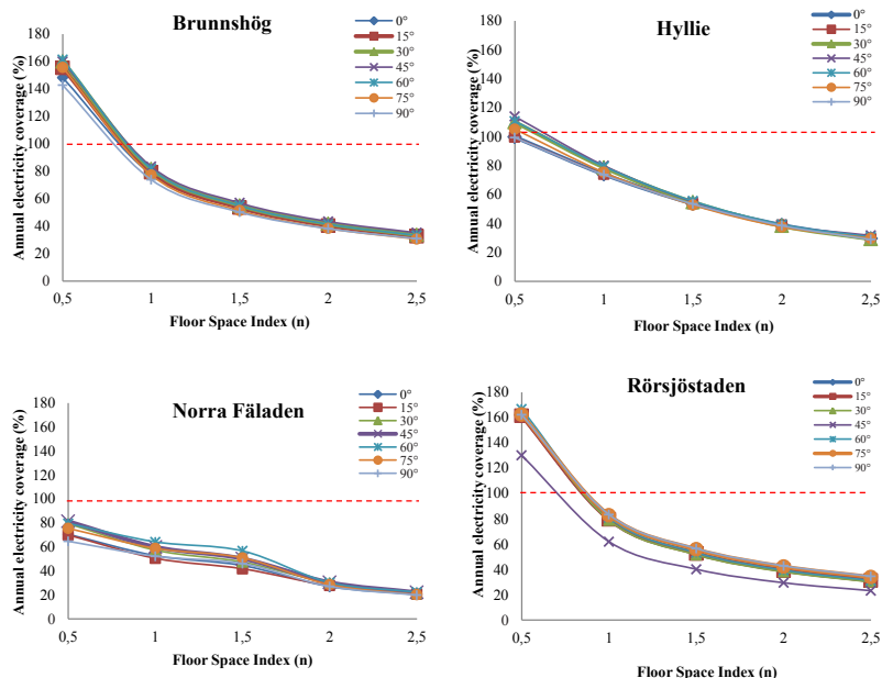
Figure 5: Annual electricity coverage at different densities
