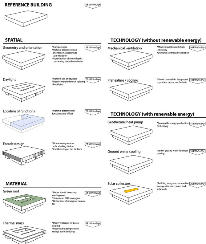
Fig. 8. Consequences of different design parameters on the energy use of a building. An example out of the design process of a Danish architect designing an office building (after Henning Larsen Architects).
