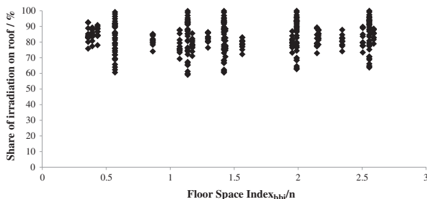
Figure 15. Share of irradiation on roof vs. density.
