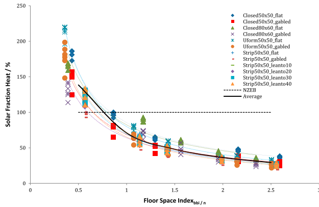
Figure 9. BBR load matching for heating demand.
