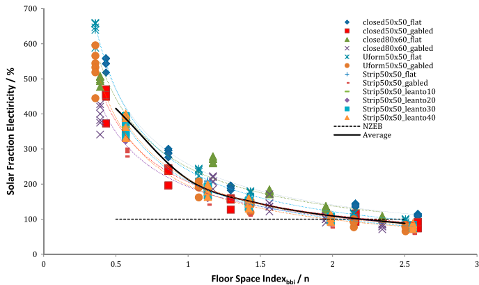
Figure 7. FEBY/BBR load matching for electricity demand.
