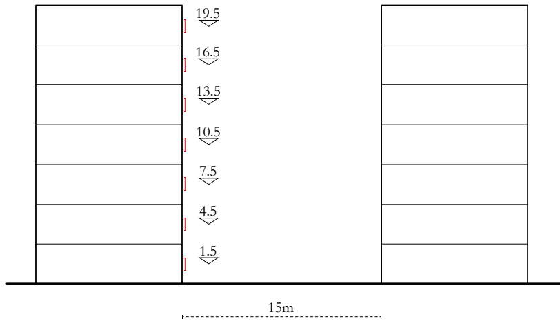
Figure 5.2 Section of building block and location of sensor points
