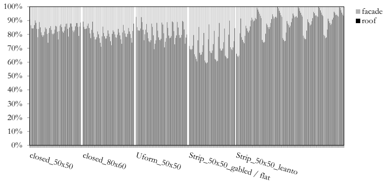
Figure 6.7 The proportion of irradiation on all suitable areas (roof and facade) per design type
