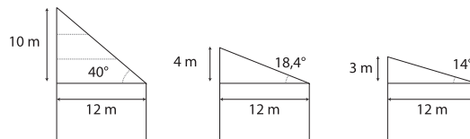
Figure 13. Consequences of roof types on building height.
