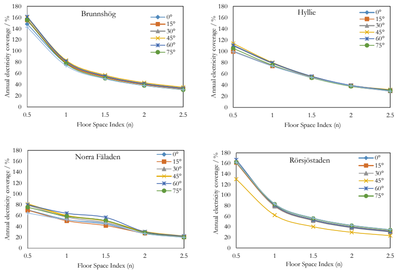
Figure 6.2 Annual electricity coverage at different densities. The different curves represent the building blocks with different orientations
