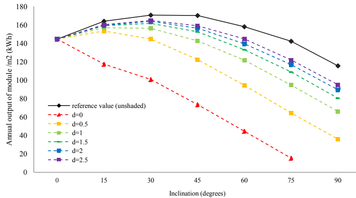
Figure 3. Output of the reference module and the shaded module in Lund.
