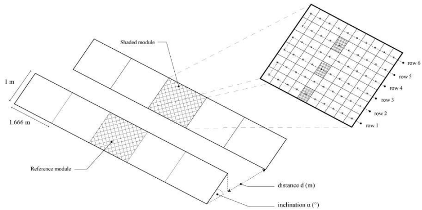
Figure 1. Layout of the two simulated rows, layout of panels / strings
