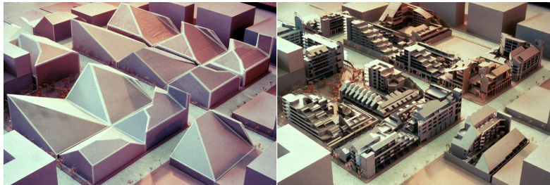
Figure 2.2 Knowles' solar envelope applied to an urban plan
