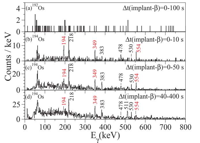
FIG. 8. (Color online) \beta -delayed \gamma -ray spectra showing transitions in (a) ^{192}\text{Os} for correlation time \Delta t(\text{implant} - \beta) = 0 \rightarrow 100 s from the decay of ^{192}\text{Re} . (b) ^{194}\text{Os} for correlation time \Delta t(\text{implant} - \beta) = 0 \rightarrow 10 s, (c) ^{194}\text{Os} for correlation time \Delta t(\text{implant} - \beta) = 0 \rightarrow 50 s, and (d) ^{194}\text{Os} for correlation time \Delta t(\text{implant} - \beta) = 40 \rightarrow 400 s, from the decay of ^{194}\text{Re} of fully stripped ions from the combination of ^{190}\text{Ta} , ^{192}\text{Ta} , and ^{194}\text{Re} settings. Previously unreported transitions are labeled in red.
