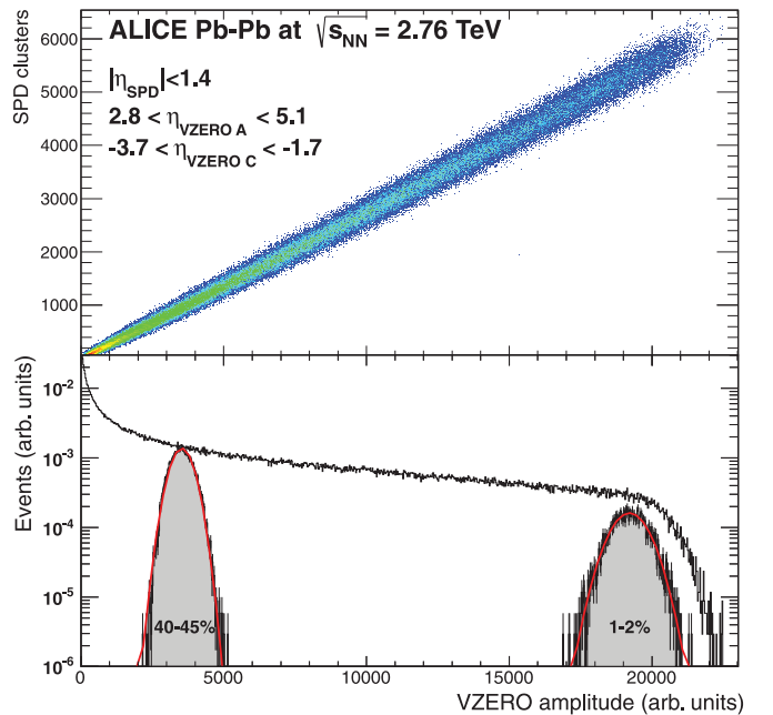
FIG. 15. (Color online) Top: Correlation between SPD multiplicity and VZERO amplitude. The rapidity coverage of each detector is indicated on the figure. Bottom: VZERO amplitude distributions for the centrality classes selected by SPD. Two centrality classes (1–2% and 40–45%) are indicated and fitted with a Gaussian.
