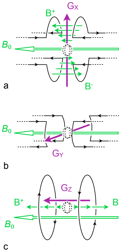
Figure 3.5 Three sets of gradient coils are built into the bore of an MRI scanner. The X and Y gradients (a and b) are similar, but aligned in different directions. Each gradient consists of two coils, generating two opposing magnetic fields ( B^+ and B^- ) which superimpose to a linear magnetic field gradient ( G_x , G_y and G_z ) through the central part of the bore, where the imaging is performed. Outside of the central part the gradient is not linear. The gradient field is in turn superimposed on the static B_0 field. By adjusting the current, the slope of the gradient is changed.
