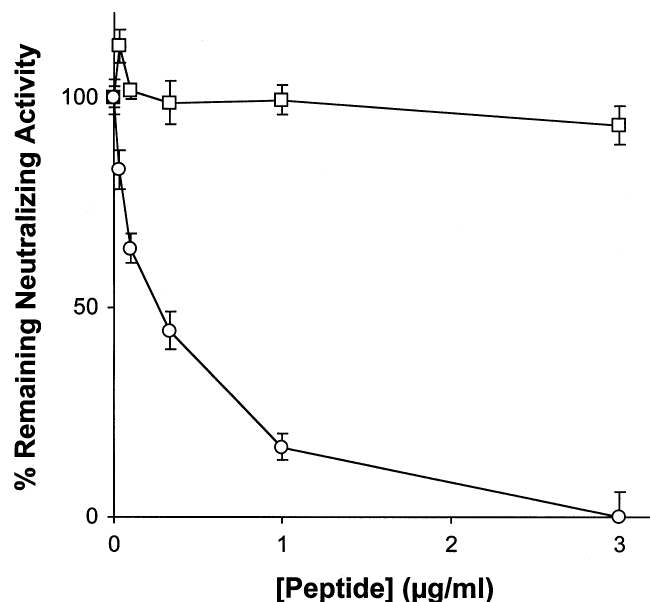
Fig. 2. Inhibition of the neutralizing activity of dimeric scFv by the addition of a soluble AD-2-mimicking peptide (○), or a negative control peptide (□). Experiments for all data points were performed in triplicate. The error bars indicate SEM.
