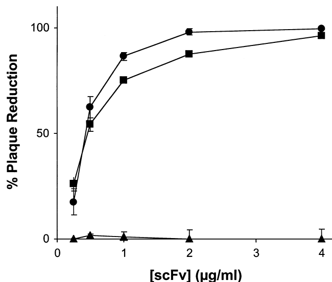
Fig. 1. Neutralization of HCMV strain AD169 infection of human embryonic lung fibroblasts in the presence of monomeric (▲) and dimeric (●) scFv, and monomeric scFv dimerized with the anti-FLAG M2 antibody (■). The plaque reduction was calculated using the Reed–Muench method (Thorpe et al. , 1987). Experiments for all data points were performed in triplicate. The error bars indicate SEM.
