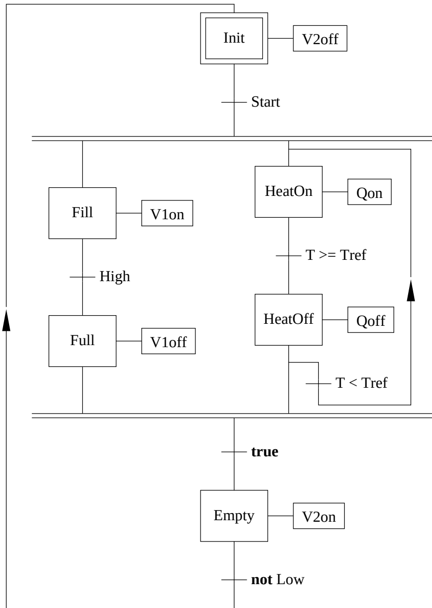
Figure 4.1 Graftet describing control of a simple boiler
