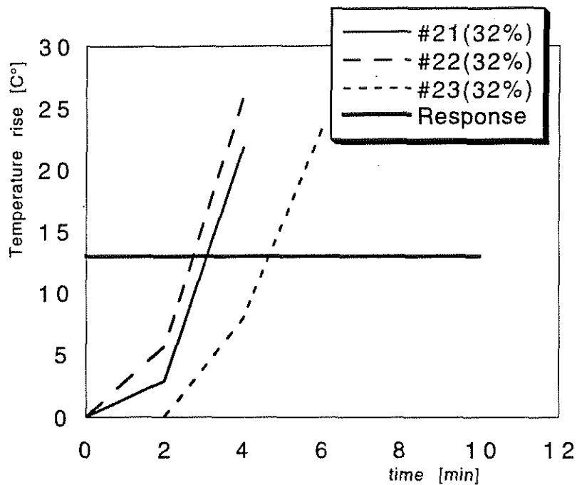
Figure 2. Temperature rise of detectors 21 - 23 located above the suspended ceiling with porosity 32%. Detectors respond at 13^\circ\text{C} temperature rise.
