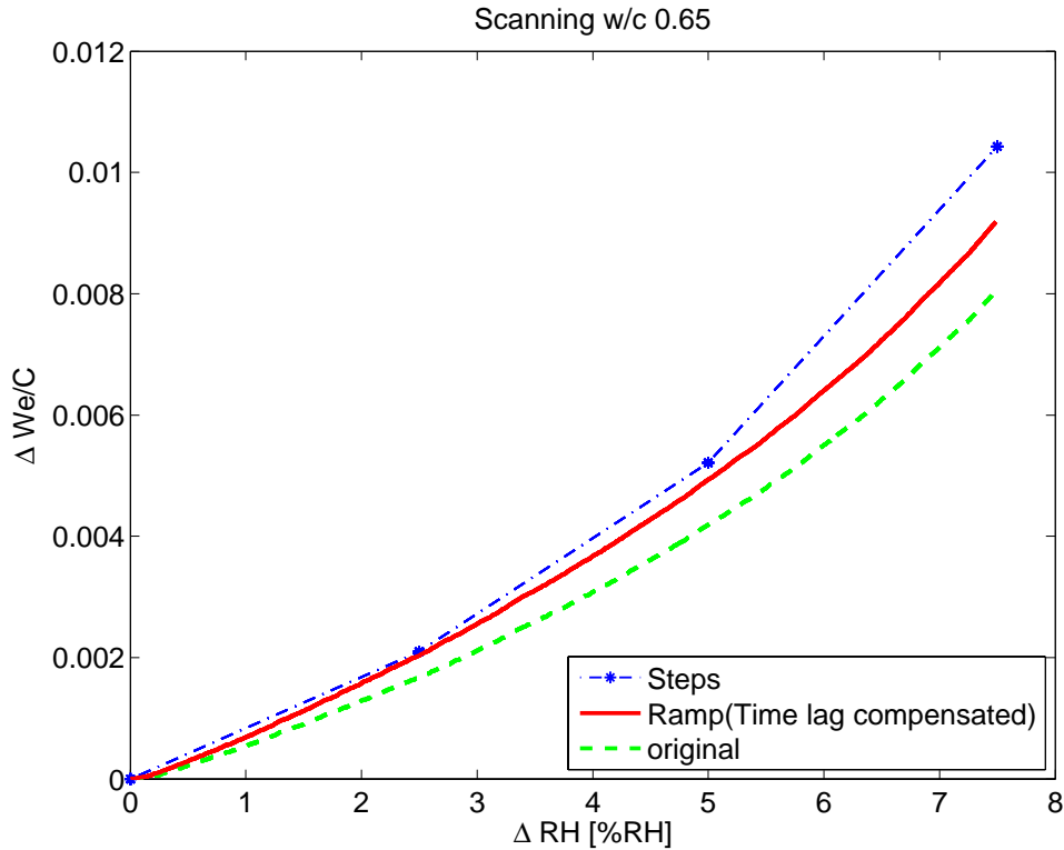
Figure 29. A comparison of the absorption scanning curves determined by using original data, a gradual RH-change (time lag compensated), and a stepwise RH-change, dashed, solid, and dash dotted line respectively. The point of origin represent the starting points at the desorption isotherm where scanning starts.
