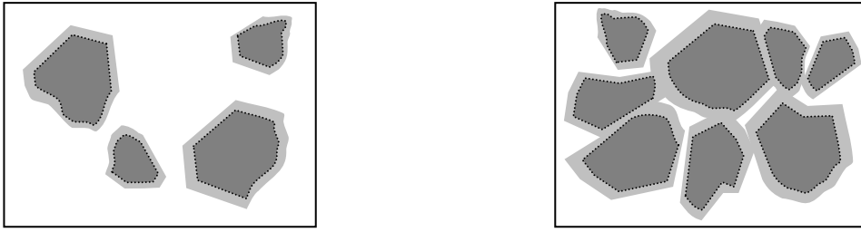
Figure 2. Illustration of a high water cement ratio to the left and a low water cement ratio to the right. Water, reaction products, CSH-gel, and cement grains are represented by the white area, lighter and darker shaded polygons respectively.
