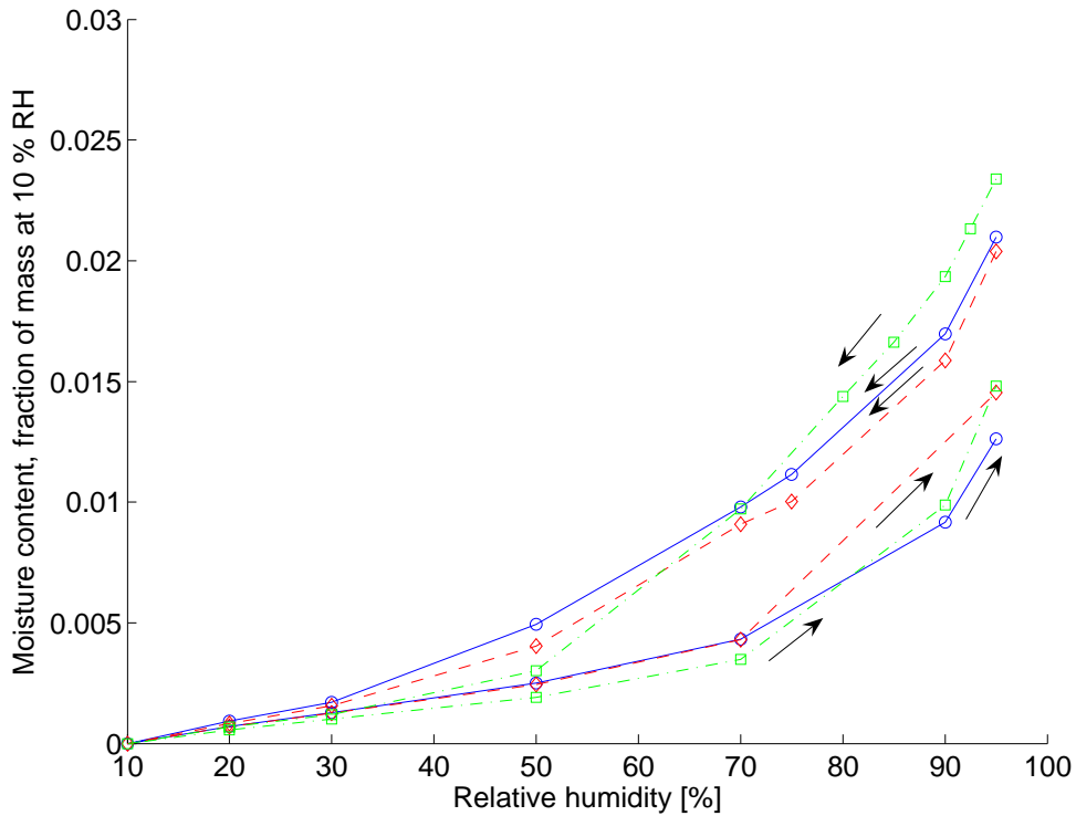
Figure 26. Sorption isotherms determined for three samples of material SFC, Floor 4310 Fibre Flow.
