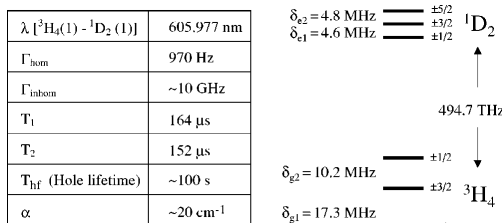
FIG. 4. Energy level diagram and relaxation data for the ^3H_4 - ^1D_2 transition of site IPr^{3+} ions in Y_2SiO_5 . T_1 , T_2 , and \Gamma_{hom} are given according to Ref. 27.
