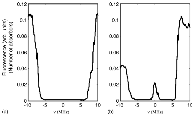
FIG. 2. Spectral hole burning in the inhomogeneously broadened {}^7F_0\text{-}{}^5D_0 transition in \text{Eu}^{3+}:\text{YAlO}_3 . The amount of \text{Eu}^{3+} ions absorbing at a particular frequency has been monitored by recording laser induced fluorescence. (a) A 12 MHz wide spectral interval has been completely emptied of absorbing ions. At laser frequencies inside the pit, the signal is constant and less than 1% of the fluorescence signal before burning. (b) An ensemble of ions has been moved back into the pit by shifting the laser frequency 69 MHz from the center of the pit and thus burning on an auxiliary hyperfine level in the ground state. The resolution of the spectral features in this experiment was limited by laser jitter of the order of 2 MHz.
