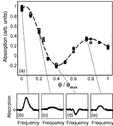
FIG. 10. Coherent driving of the \pm 1/2-\pm 3/2 transition. Pulses with a variable pulse area ( \theta=\Omega t ) was applied to the transition using 3\ \mu\text{s} long pulses with varying intensity. The population difference between the ground [ \pm 1/2(g) ] and optically excited [ \pm 3/2(e) ] states, after the pulse, was monitored by recording the transmission at the resonance frequency. (b)–(e) An ensemble of ions absorbing/emitting on the transition after the application of a pulse with (b) \theta=0 , (c) \theta\approx\pi/3 , (d) \theta\approx\pi , and (e) \theta\approx 2\pi .
