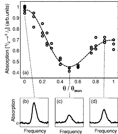
FIG. 11. Coherent driving of the \pm 5/2-\pm 1/2 transition. Pulses with a variable pulse area ( \theta=\Omega t ) was applied to the transition using 3\ \mu\text{s} long pulses with varying intensity. The number of ions left in the ground state, \pm 5/2(g) , after the pulse, was monitored by recording the absorption on the \pm 5/2-\pm 5/2 transition. (b)–(d) An ensemble of ions absorbing on \pm 5/2-\pm 5/2 after the application of a pulse with (b) \theta=0 , (c) \theta\approx\pi , and (d) \theta\approx 2\pi , resonant with \pm 5/2-\pm 1/2 .
