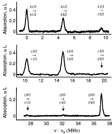
FIG. 7. Ions absorbing on specific hyperfine transitions, inside the inhomogeneously broadened {}^3H_4 - {}^1D_2 transition in Pr^{3+}:Y_2SiO_5 . The three curves correspond to three separate experiments. The three peaks of varying size, in each curve, are due to the same ensemble of ions absorbing on different transitions. The intensity was attenuated by a factor 10^3 during readout, in order not to cause significant excitation when probing the transitions. The scan rate during readout was of the order of r \approx 0.1 MHz/ \mu s. Single-shot measurements.
