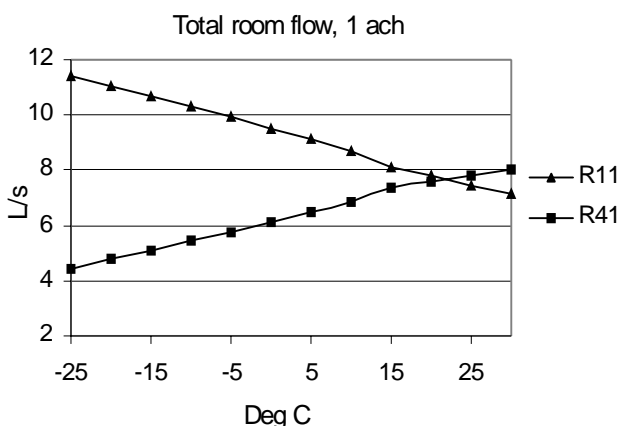
Fig. 5 Air flows through infiltration and supply air device to room 11 at floor 1 and room 41 at floor 4
