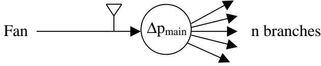
Fig.8. Schematic figure of a supply air system. The static pressure is set after the fan because there is a pressure loss in the main duct when the flow is divided to the branches. The branches have a constant static pressure.
