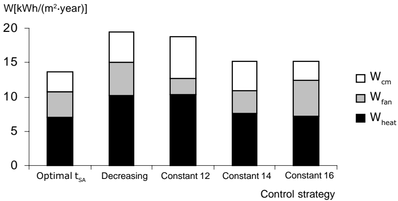
Fig. 7. Energy use per m² floor area for one zone with a facade area of 9 m² and a floor area of 13.5 m² during one year (1977) in daytime in Sturup with a constant internal heat load of 26 W/m² floor area. The average U-value of the building envelope is 1.5 W/(m²·°C) and no infiltration is assumed. W_{cm} is energy used by the chiller, W_{fan} is energy used by the fan and W_{heat} is energy used to heat the air either in the room or in the HVAC unit. Solar radiation is not included.
