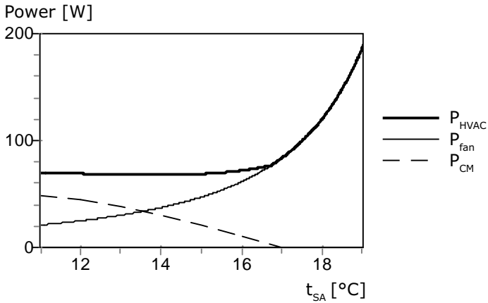
Fig. 13. The power requirement ( P_{HVAC} ) depending on supply air temperature in Case 3 at 16°C outdoor temperature. Input data according to Fig. 11.
