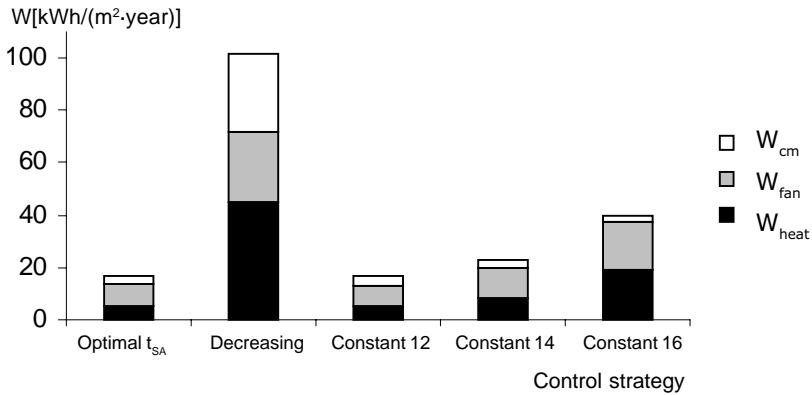
Fig. 21. Day time energy use per m 2 floor area for one zone with a facade area of 9 m 2 during one year in Luleå with an internal load of 600 W (corresponding to 44 W/m 2 floor area).
