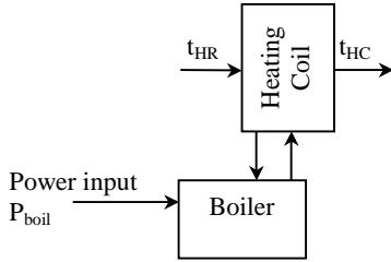
Fig. 3. Boiler and heating coil.
