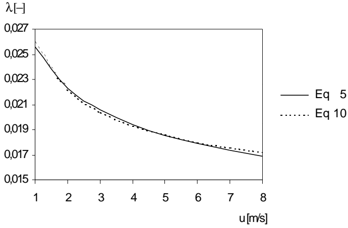
Fig. 6. Friction loss coefficient \lambda as a function of air velocity ( d=0.315 m \lambda_0=0.0257 m 0.2 /s 0.2 ) depending on Eq. (5) and Eq. (10).
