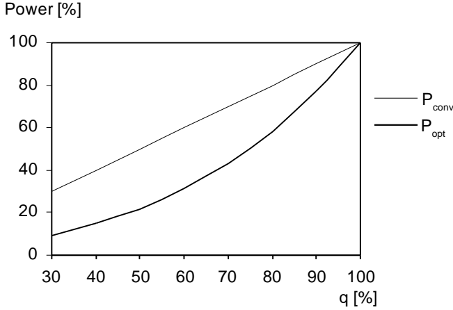
Fig. 17. The power required to transport the air through the duct system, i.e. immediately after the HVAC unit to the room. P_{opt} is the power used with optimized static pressure set point and P_{conv} is without the optimization.
