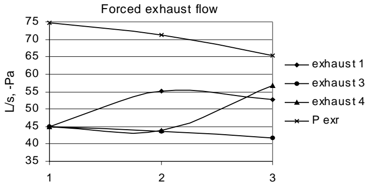
Fig. 9 Total exhaust flows and pressure before the filter (P extr)
