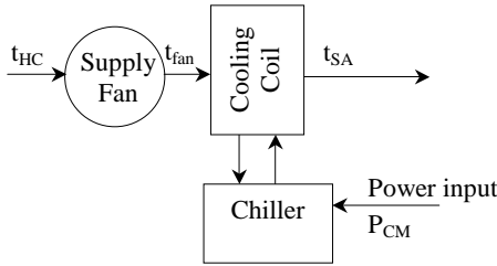
Fig. 4. Chiller and cooling coil.
