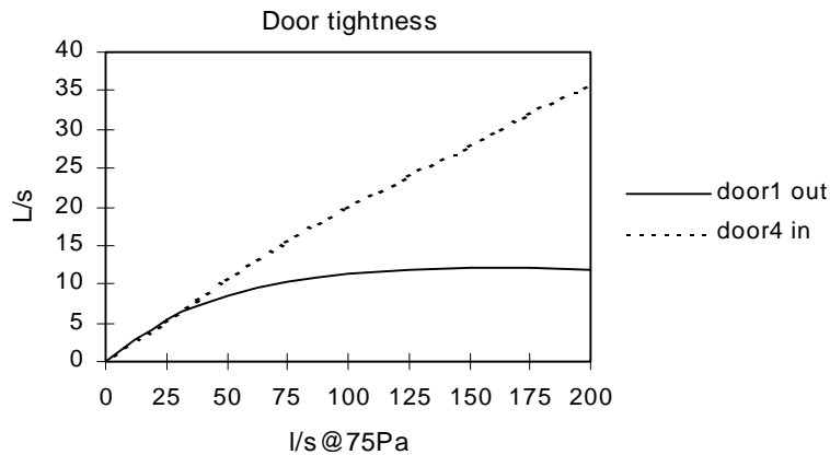
Fig. 7 The airflow out of apartment 1 through door 1 and the airflow into apartment 4 through door 4 at different levels of tightness at -10°C outdoors
