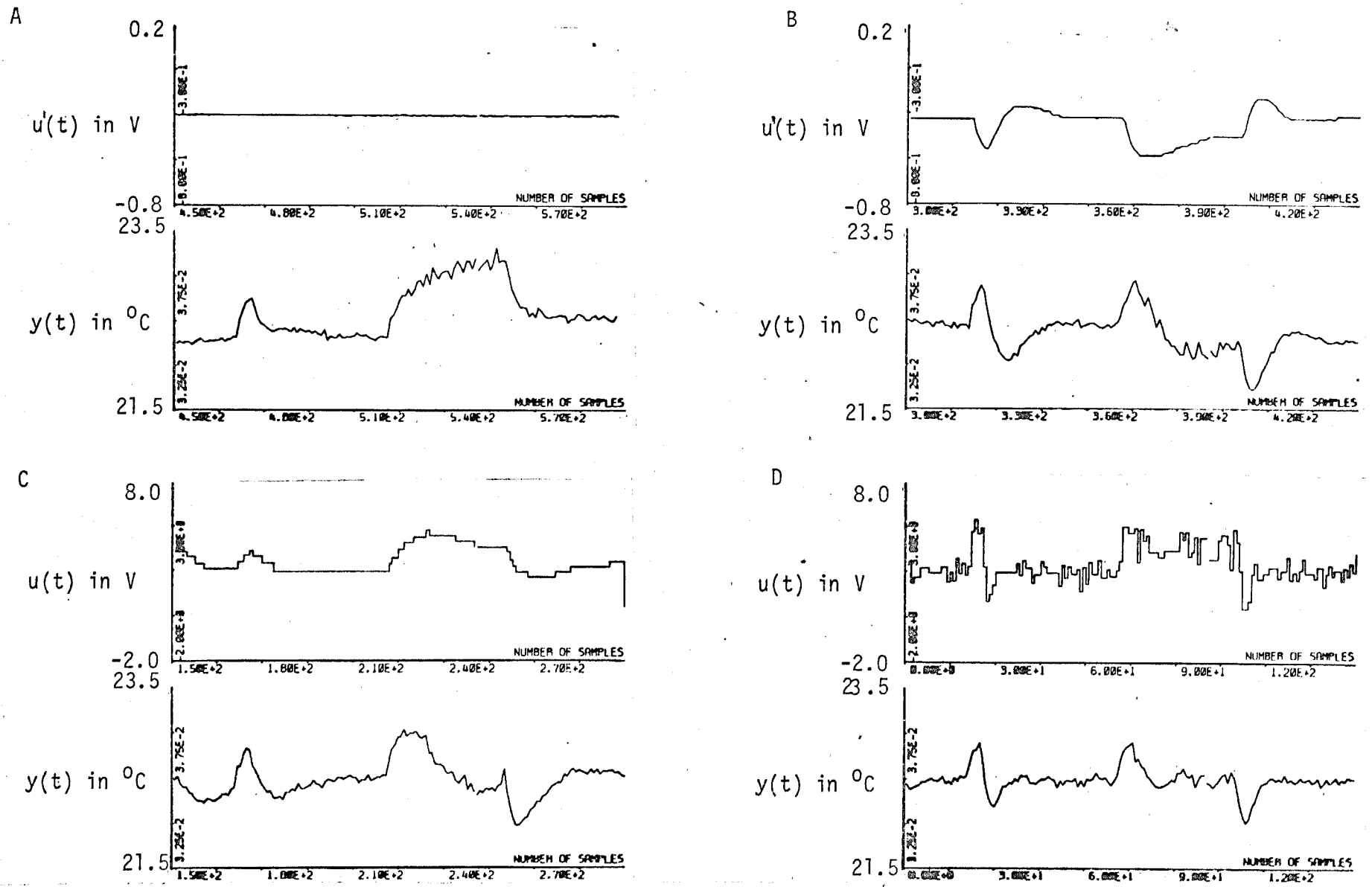
Fig 3. Climate control. Full scale experiments with a heat load of 2 kW. u(t) is the control signal in volts and u'(t) is the position of the valve in volts ( u'(t) \approx -0.1 u(t) ). y(t) is the air temperature after the room in °C.
