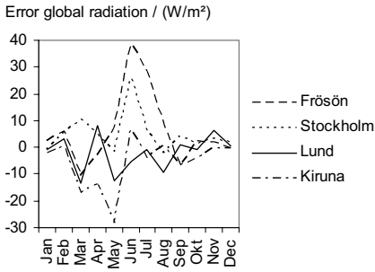
Figure 32. The error in monthly average global radiation as the simulated value minus the measured.
