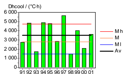
Figure 14. Annual degree hours for cooling for the readings for each year respectively together with the average from the extreme and normal years of Meteororm for Lund.
