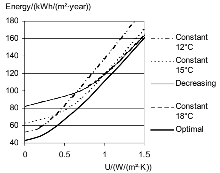
Figure 17. The annual total energy use (without energy for internal heat) depending on U-value of the area towards outdoors. The calculation was made for Frösön and the office zone was occupied between 08.00 and 18.00.
