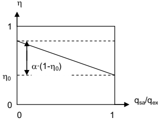
Figure 2. The temperature efficiency of the heat recovery unit based on the supply side as a function of the under-balance.
