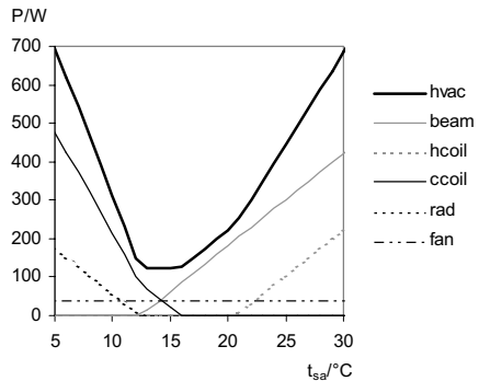
Figure 8. The different power used by the HVAC system in the example for 15^\circ\text{C} outdoor temperature. To the right, P_{beam} and P_{hcoil} is positive and P_{coil} and P_{rad} is zero. At 12^\circ\text{C} , condensation starts in the supply air with a change in the derivative of the P_{coil} .
