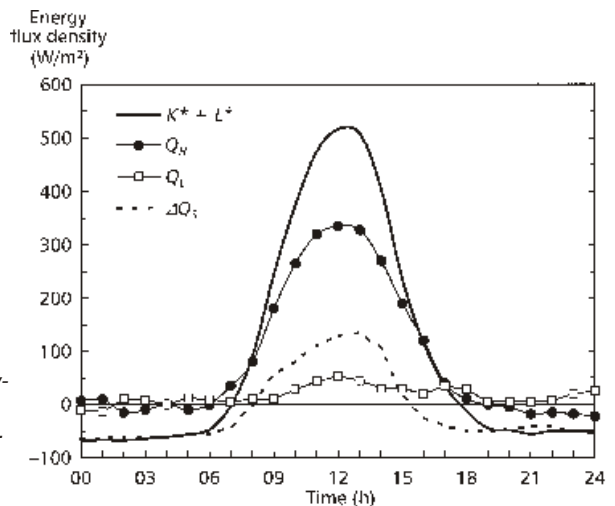
Fig. 3.6 The energy balance according to equation 3.5 for an urban canyon in Vancouver, Canada. K^* + L^* = net short and long-wave radiation, Q_H = sensible heat, Q_E = latent heat and DQ_S = heat storage. The anthropogenic heat Q_F and advection DQ_A were not measured and are included in the other heat fluxes. They are, however, assumed to be small. (Modified after Oke 1987).
