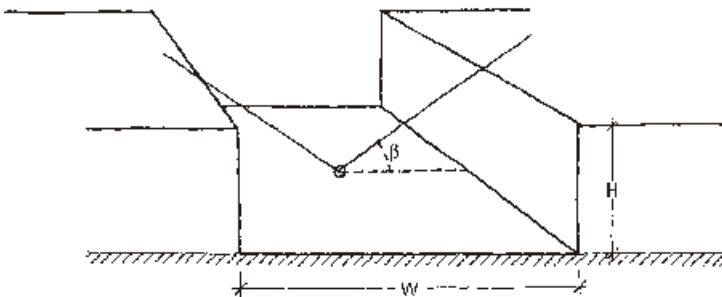
Fig. 3.3 Sky view factor of an urban street canyon. At the middle of the street of an infinitely long canyon, SVF = \cos \beta .
