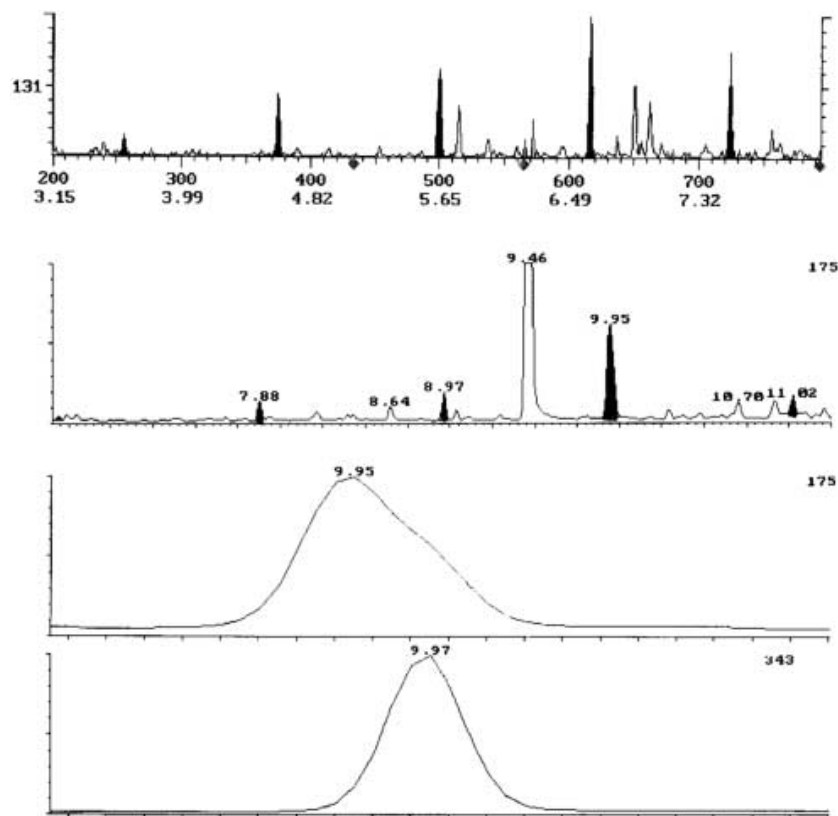
Fig. 1 Analysis of 3-hydroxy fatty acids of 10, 12, 14, 16, and 18 carbon chain lengths (blackened) in a dust sample by using GC-MSMS focusing at m/z 131 and GC-MS focusing at m/z 175 (upper two tracings); detail of the region of 3-hydroxyhexadecanoic acid in the same sample preparation achieved by using GC-MS focusing at m/z 175 and m/z 343 (lower two tracings). Abscissa: minutes; ordinate: relative ion intensity
